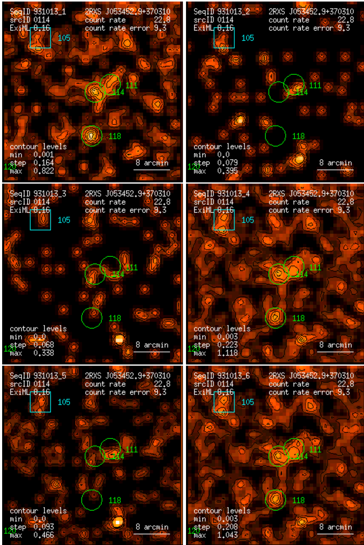
Figure 114: RASS 931013: detection 0114: band rate images, Gaussian filter: (1) PSPC channels 11 – 41, (2) 52 – 90, (3) 91 – 201, (4) 11 – 235, (5) 52 – 201, (6) 11 – 201. Broad band rates in counts/ks. Band rate contour levels in counts/ks/arcmin 2 .
