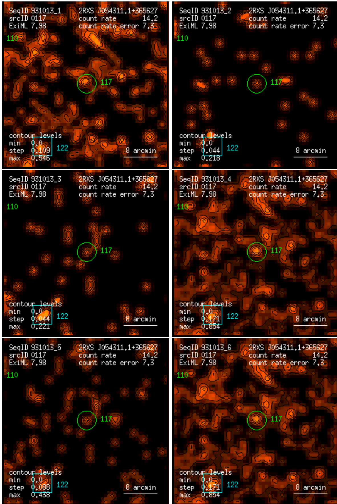
Figure 117: RASS 931013: detection 0117: band rate images, Gaussian filter: (1) PSPC channels 11 – 41, (2) 52 – 90, (3) 91 – 201, (4) 11 – 235, (5) 52 – 201, (6) 11 – 201. Broad band rates in counts/ks. Band rate contour levels in counts/ks/arcmin 2 .
