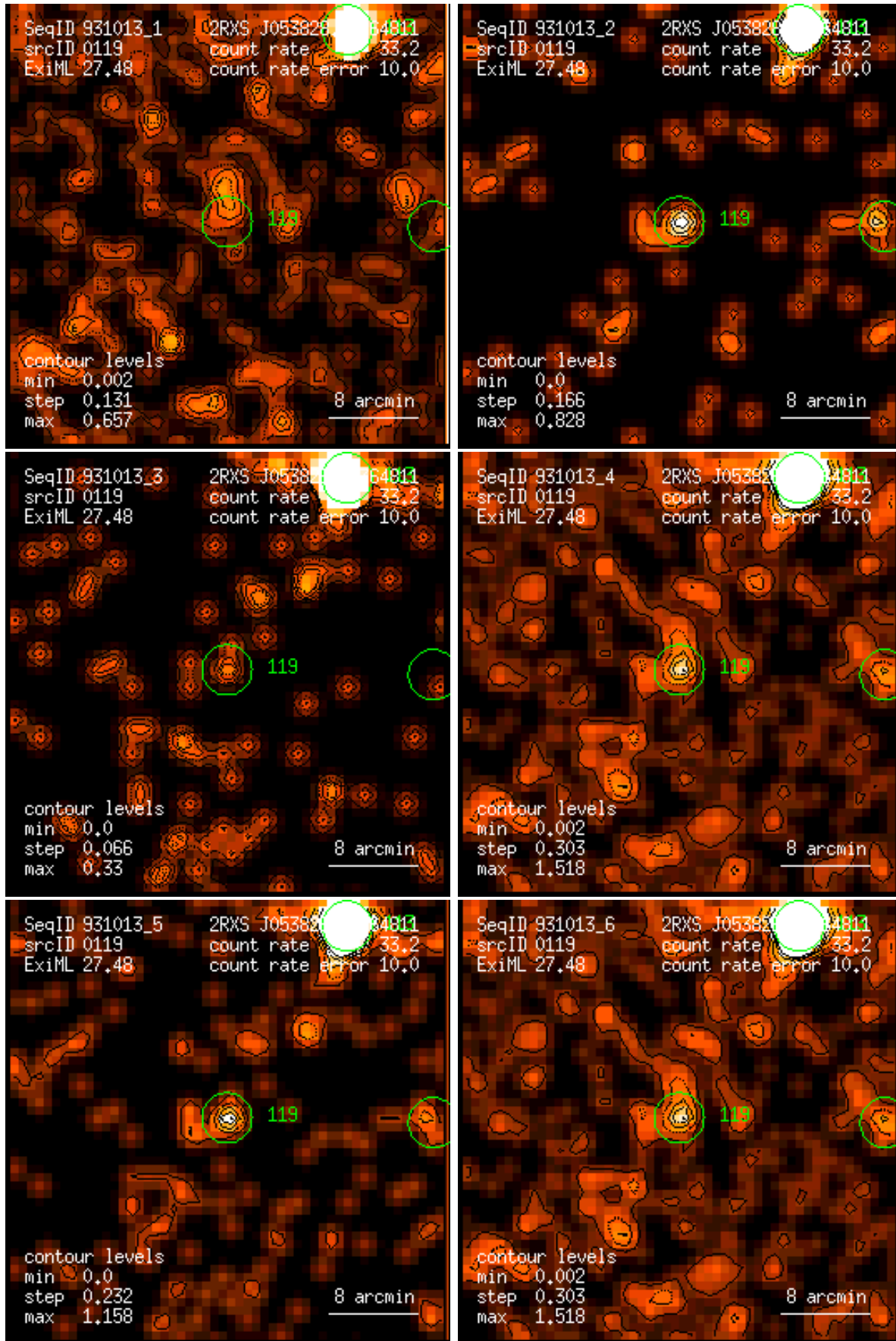
Figure 119: RASS 931013: detection 0119: band rate images, Gaussian filter: (1) PSPC channels 11 – 41, (2) 52 – 90, (3) 91 – 201, (4) 11 – 235, (5) 52 – 201, (6) 11 – 201. Broad band rates in counts/ks. Band rate contour levels in counts/ks/arcmin 2 .
