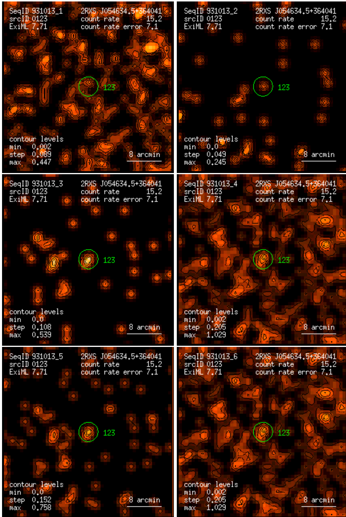
Figure 123: RASS 931013: detection 0123: band rate images, Gaussian filter: (1) PSPC channels 11 – 41, (2) 52 – 90, (3) 91 – 201, (4) 11 – 235, (5) 52 – 201, (6) 11 – 201. Broad band rates in counts/ks. Band rate contour levels in counts/ks/arcmin 2 .
