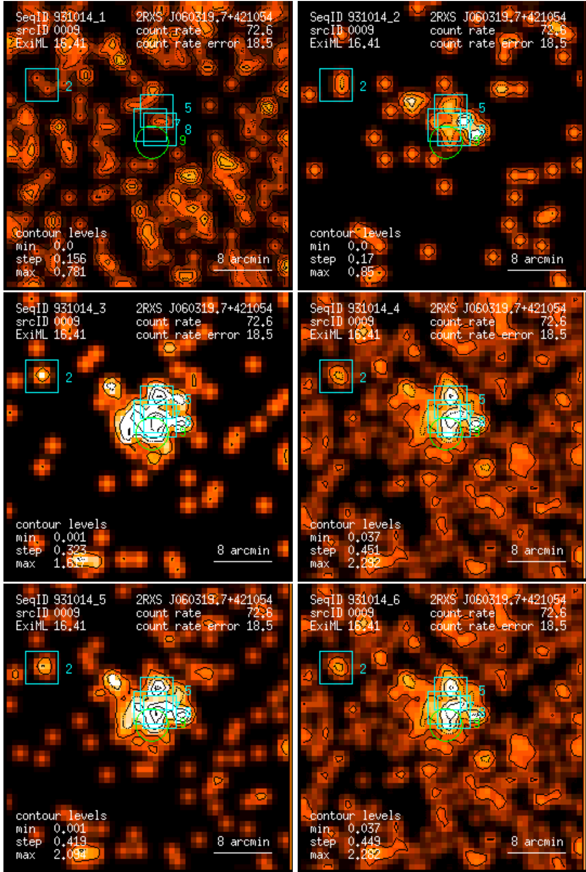
Figure 9: RASS 931014: detection 0009: band rate images, Gaussian filter: (1) PSPC channels 11 – 41, (2) 52 – 90, (3) 91 – 201, (4) 11 – 235, (5) 52 – 201, (6) 11 – 201. Broad band rates in counts/ks. Band rate contour levels in counts/ks/arcmin 2 .
