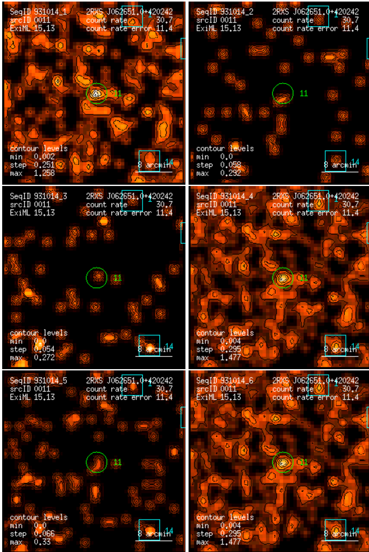
Figure 11: RASS 931014: detection 0011: band rate images, Gaussian filter: (1) PSPC channels 11 – 41, (2) 52 – 90, (3) 91 – 201, (4) 11 – 235, (5) 52 – 201, (6) 11 – 201. Broad band rates in counts/ks. Band rate contour levels in counts/ks/arcmin 2 .
