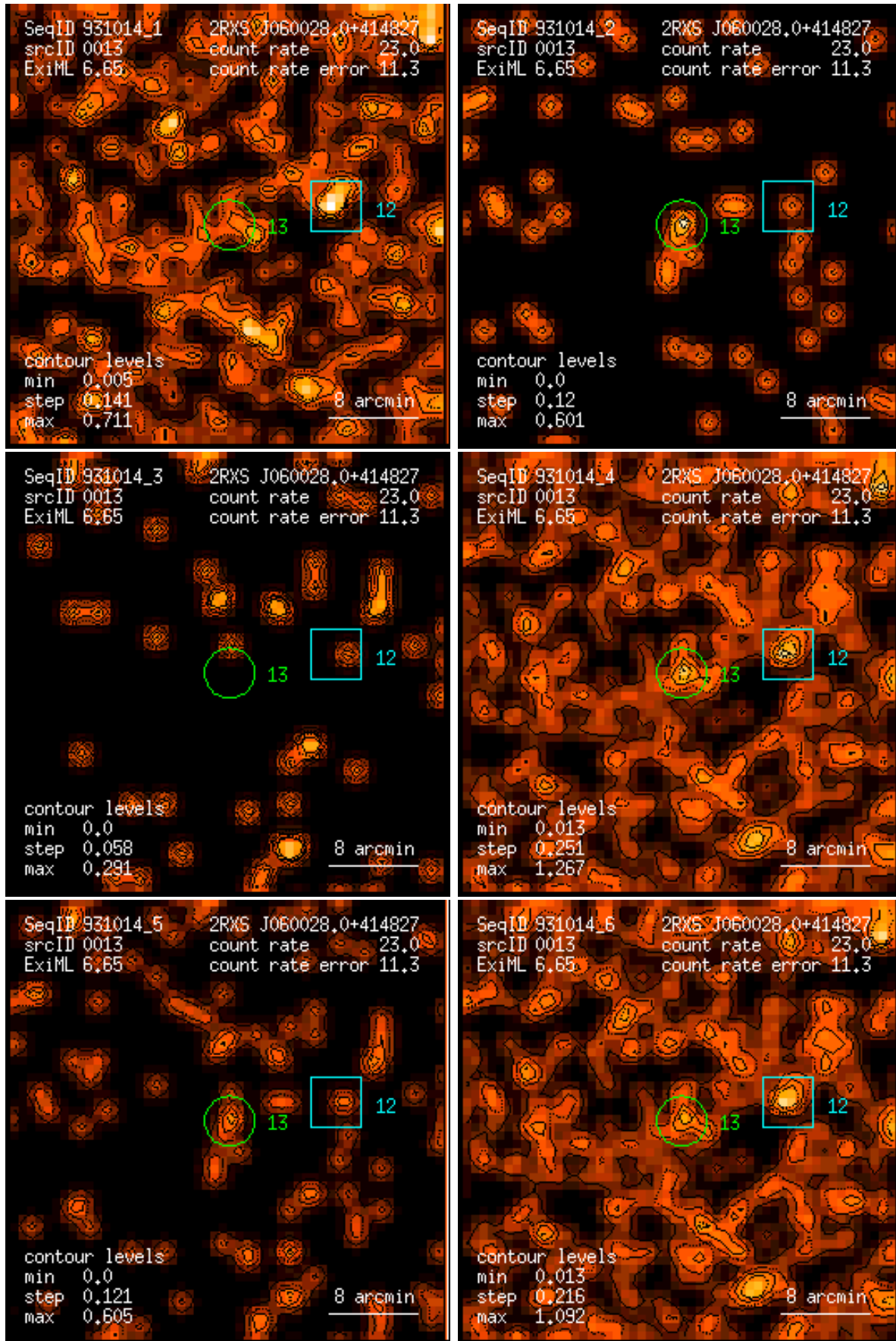
Figure 13: RASS 931014: detection 0013: band rate images, Gaussian filter: (1) PSPC channels 11 – 41, (2) 52 – 90, (3) 91 – 201, (4) 11 – 235, (5) 52 – 201, (6) 11 – 201. Broad band rates in counts/ks. Band rate contour levels in counts/ks/arcmin 2 .
