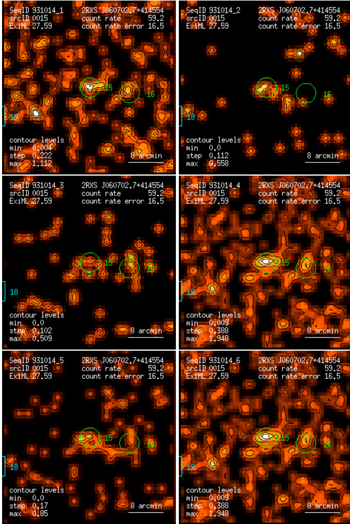
Figure 15: RASS 931014: detection 0015: band rate images, Gaussian filter: (1) PSPC channels 11 – 41, (2) 52 – 90, (3) 91 – 201, (4) 11 – 235, (5) 52 – 201, (6) 11 – 201. Broad band rates in counts/ks. Band rate contour levels in counts/ks/arcmin 2 .
