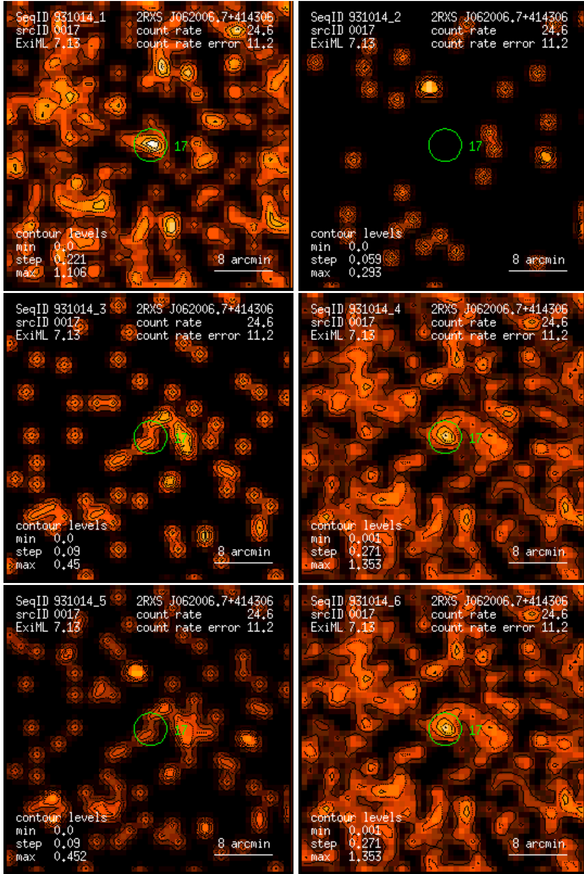
Figure 17: RASS 931014: detection 0017: band rate images, Gaussian filter: (1) PSPC channels 11 – 41, (2) 52 – 90, (3) 91 – 201, (4) 11 – 235, (5) 52 – 201, (6) 11 – 201. Broad band rates in counts/ks. Band rate contour levels in counts/ks/arcmin 2 .
