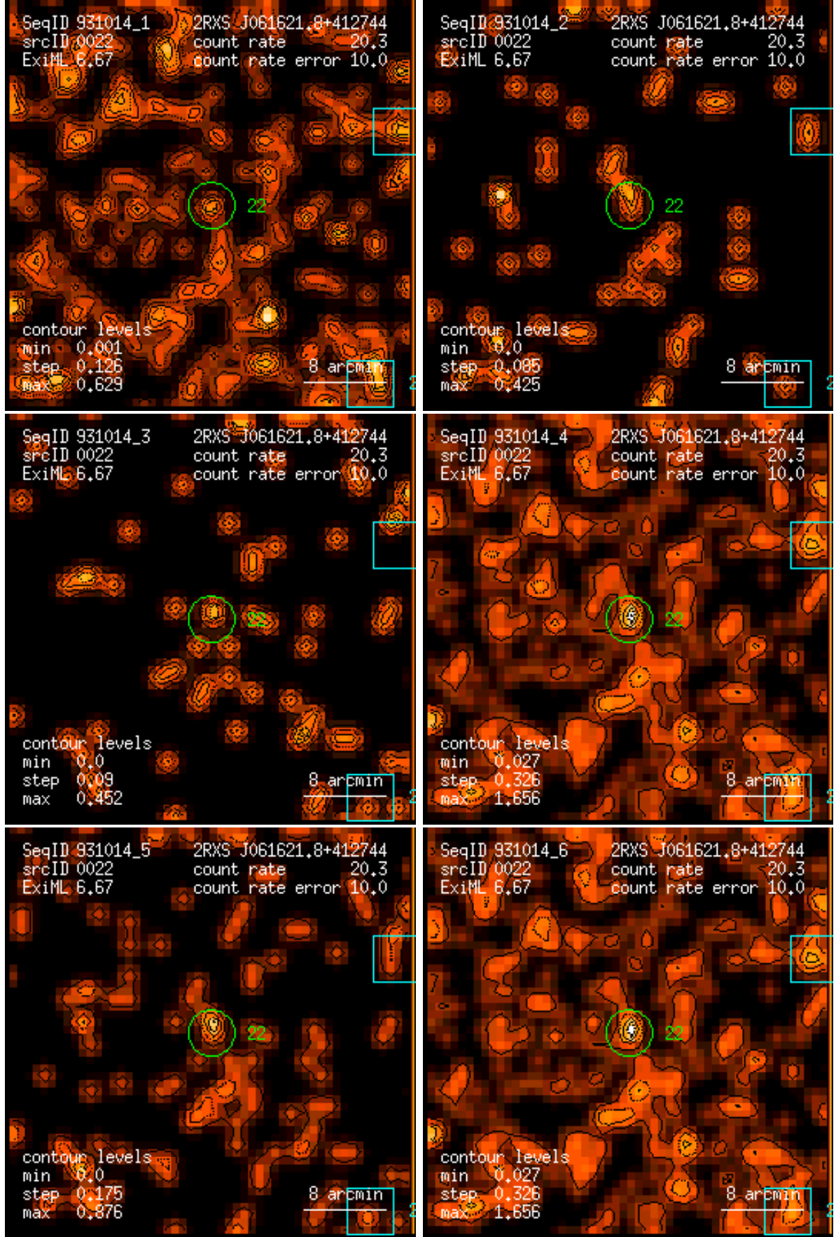
Figure 22: RASS 931014: detection 0022: band rate images, Gaussian filter: (1) PSPC channels 11 – 41, (2) 52 – 90, (3) 91 – 201, (4) 11 – 235, (5) 52 – 201, (6) 11 – 201. Broad band rates in counts/ks. Band rate contour levels in counts/ks/arcmin 2 .
