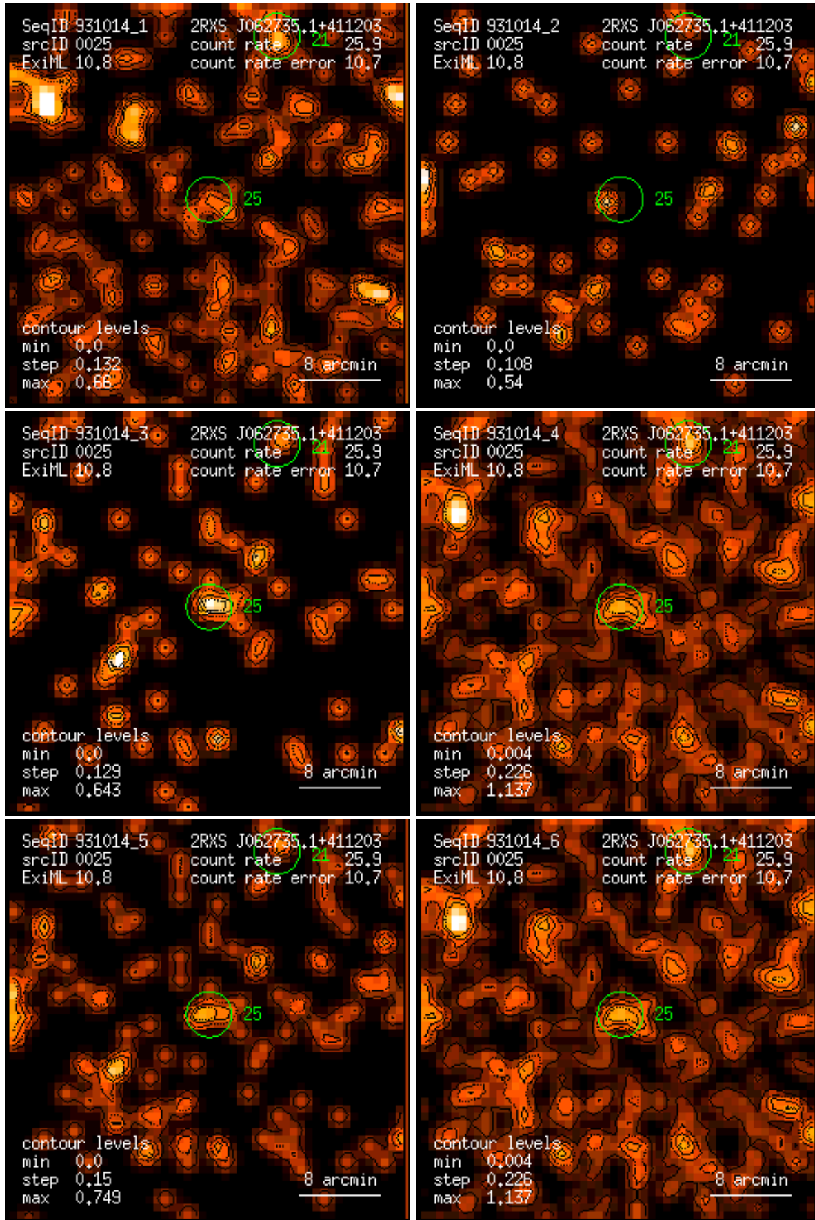
Figure 25: RASS 931014: detection 0025: band rate images, Gaussian filter: (1) PSPC channels 11 – 41, (2) 52 – 90, (3) 91 – 201, (4) 11 – 235, (5) 52 – 201, (6) 11 – 201. Broad band rates in counts/ks. Band rate contour levels in counts/ks/arcmin 2 .
