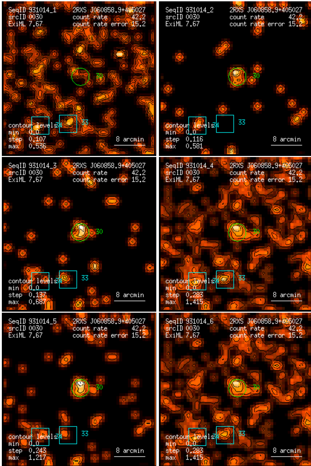
Figure 30: RASS 931014: detection 0030: band rate images, Gaussian filter: (1) PSPC channels 11 – 41, (2) 52 – 90, (3) 91 – 201, (4) 11 – 235, (5) 52 – 201, (6) 11 – 201. Broad band rates in counts/ks. Band rate contour levels in counts/ks/arcmin 2 .
