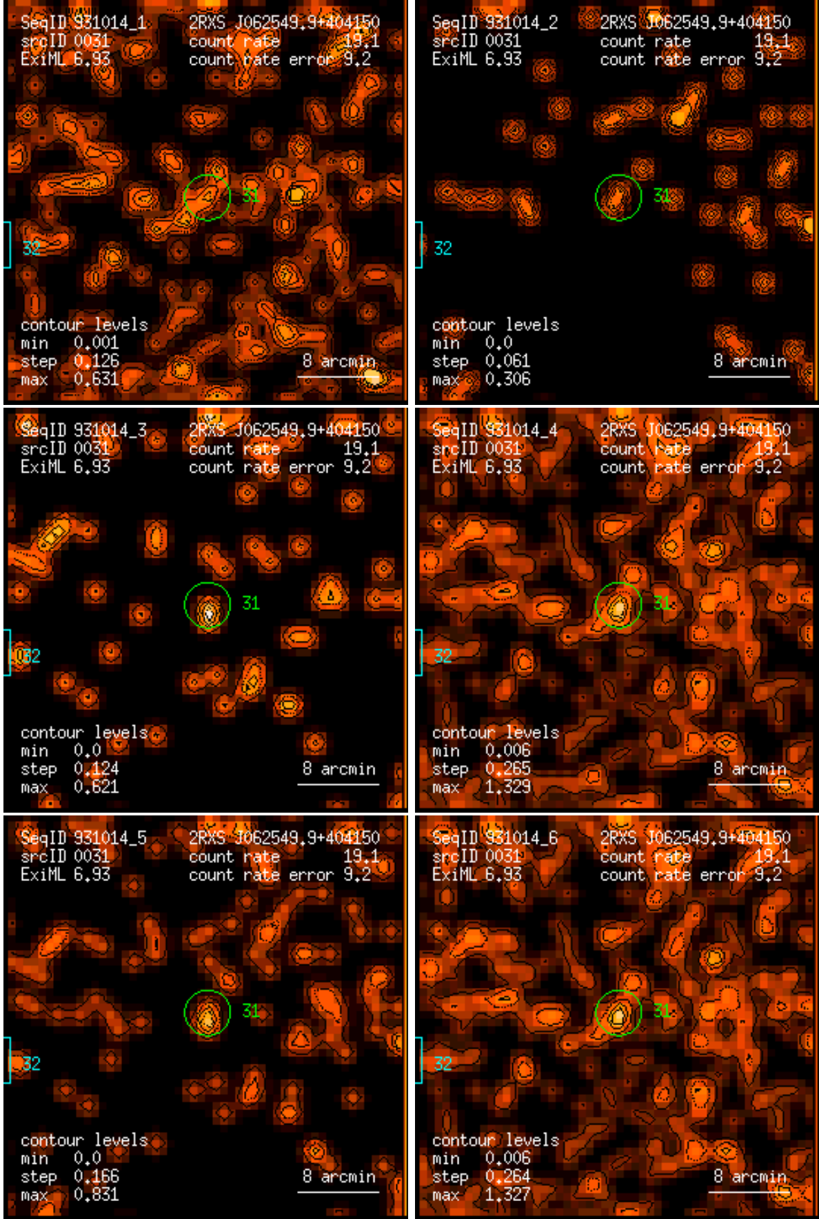
Figure 31: RASS 931014: detection 0031: band rate images, Gaussian filter: (1) PSPC channels 11 – 41, (2) 52 – 90, (3) 91 – 201, (4) 11 – 235, (5) 52 – 201, (6) 11 – 201. Broad band rates in counts/ks. Band rate contour levels in counts/ks/arcmin 2 .
