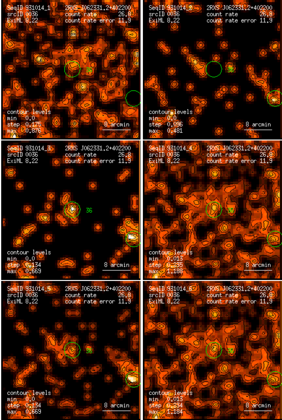
Figure 36: RASS 931014: detection 0036: band rate images, Gaussian filter: (1) PSPC channels 11 – 41, (2) 52 – 90, (3) 91 – 201, (4) 11 – 235, (5) 52 – 201, (6) 11 – 201. Broad band rates in counts/ks. Band rate contour levels in counts/ks/arcmin 2 .
