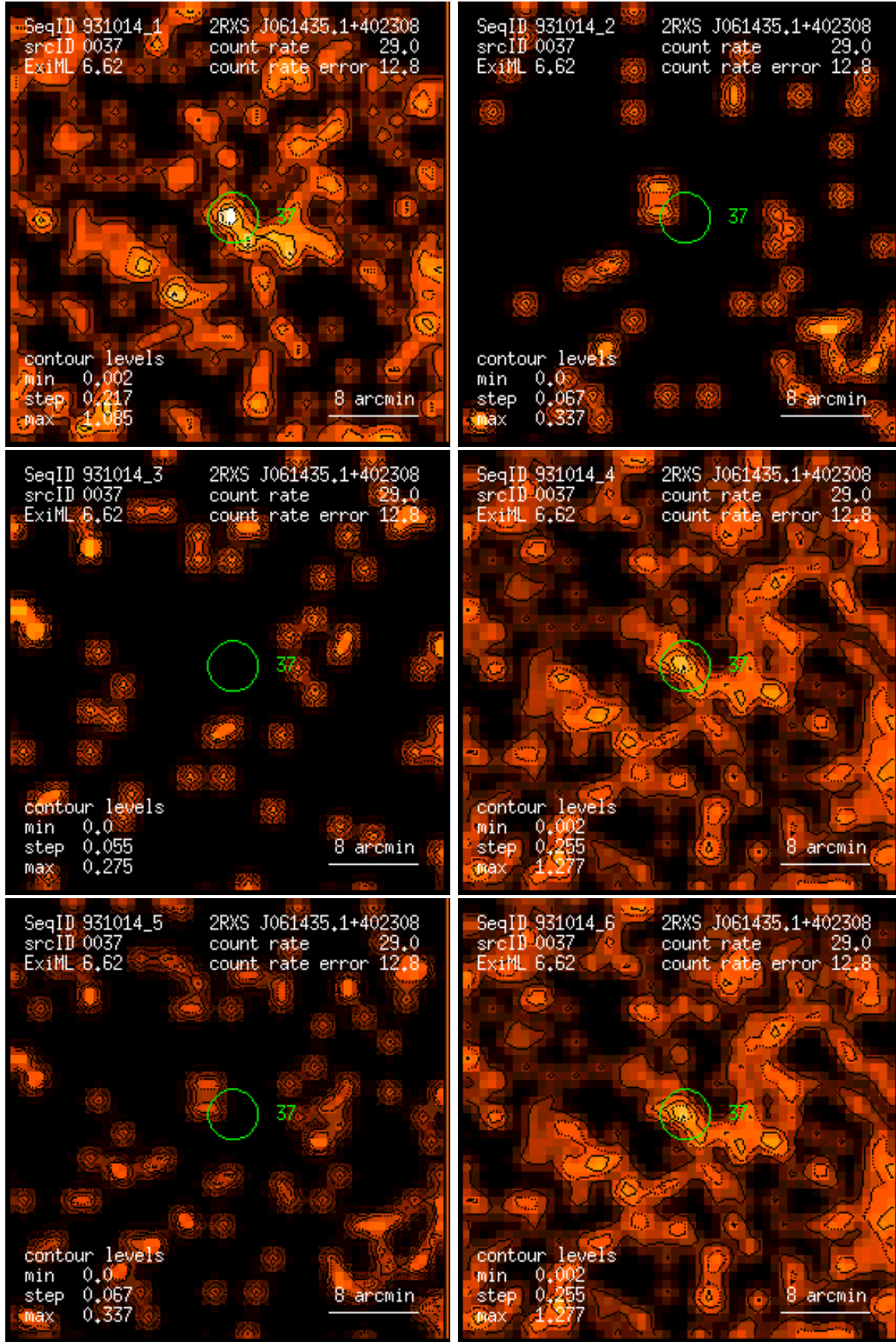
Figure 37: RASS 931014: detection 0037: band rate images, Gaussian filter: (1) PSPC channels 11 – 41, (2) 52 – 90, (3) 91 – 201, (4) 11 – 235, (5) 52 – 201, (6) 11 – 201. Broad band rates in counts/ks. Band rate contour levels in counts/ks/arcmin 2 .
