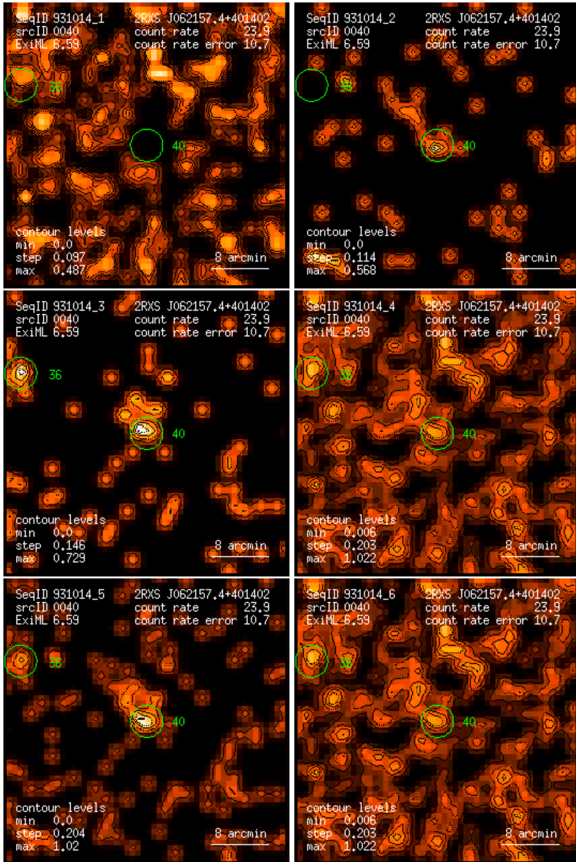
Figure 40: RASS 931014: detection 0040: band rate images, Gaussian filter: (1) PSPC channels 11 – 41, (2) 52 – 90, (3) 91 – 201, (4) 11 – 235, (5) 52 – 201, (6) 11 – 201. Broad band rates in counts/ks. Band rate contour levels in counts/ks/arcmin 2 .
