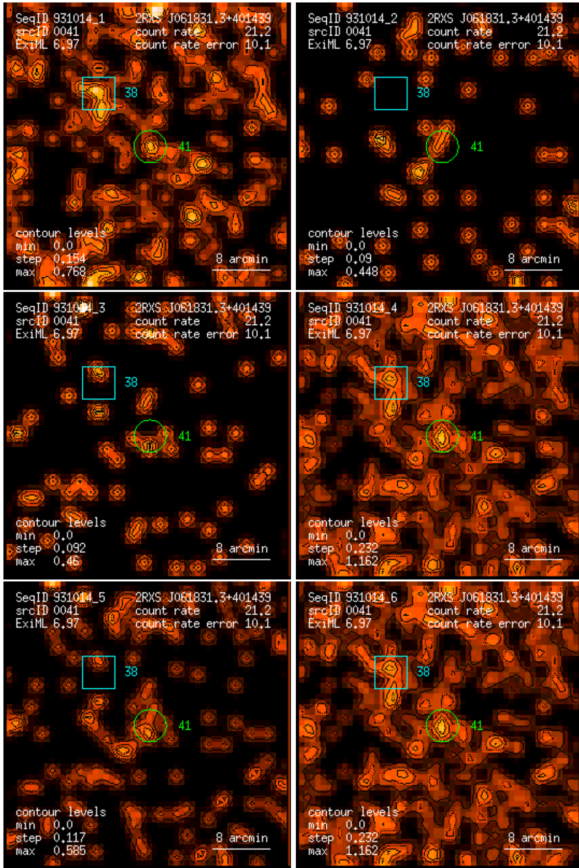
Figure 41: RASS 931014: detection 0041: band rate images, Gaussian filter: (1) PSPC channels 11 – 41, (2) 52 – 90, (3) 91 – 201, (4) 11 – 235, (5) 52 – 201, (6) 11 – 201. Broad band rates in counts/ks. Band rate contour levels in counts/ks/arcmin 2 .
