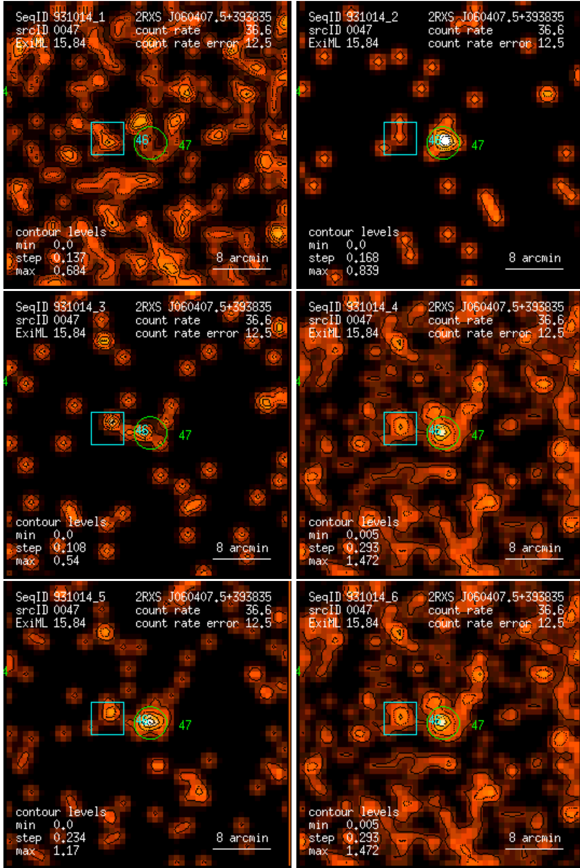
Figure 47: RASS 931014: detection 0047: band rate images, Gaussian filter: (1) PSPC channels 11 – 41, (2) 52 – 90, (3) 91 – 201, (4) 11 – 235, (5) 52 – 201, (6) 11 – 201. Broad band rates in counts/ks. Band rate contour levels in counts/ks/arcmin 2 .
