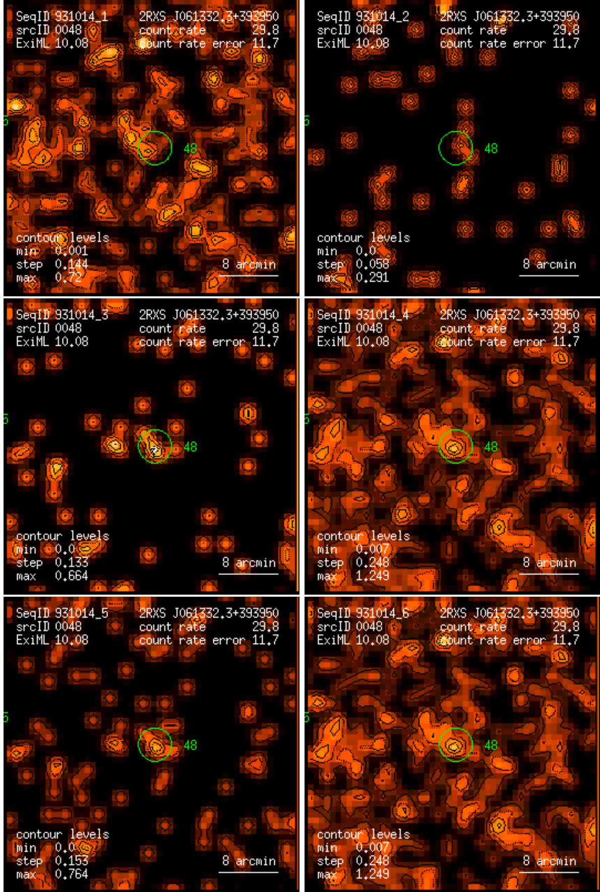
Figure 48: RASS 931014: detection 0048: band rate images, Gaussian filter: (1) PSPC channels 11 – 41, (2) 52 – 90, (3) 91 – 201, (4) 11 – 235, (5) 52 – 201, (6) 11 – 201. Broad band rates in counts/ks. Band rate contour levels in counts/ks/arcmin 2 .
