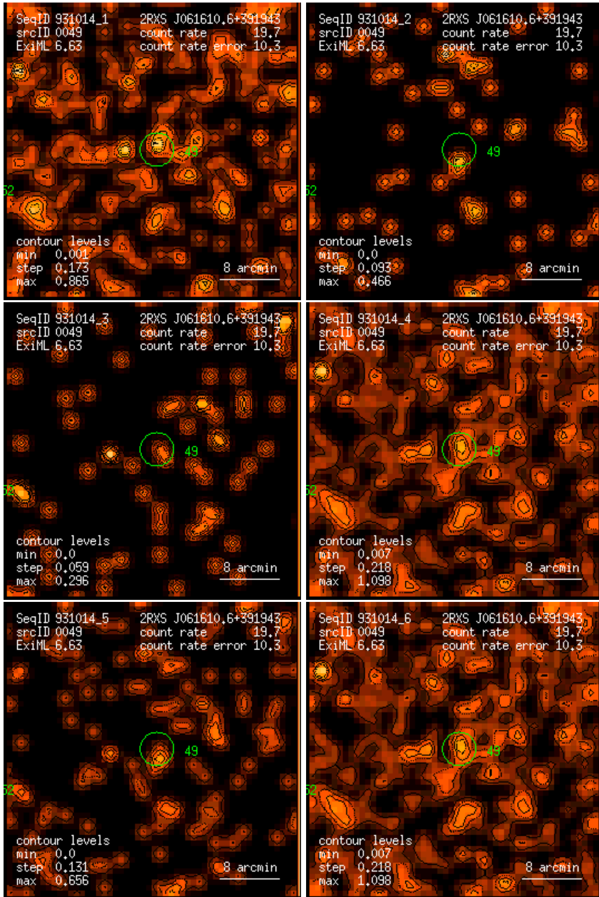
Figure 49: RASS 931014: detection 0049: band rate images, Gaussian filter: (1) PSPC channels 11 – 41, (2) 52 – 90, (3) 91 – 201, (4) 11 – 235, (5) 52 – 201, (6) 11 – 201. Broad band rates in counts/ks. Band rate contour levels in counts/ks/arcmin 2 .
