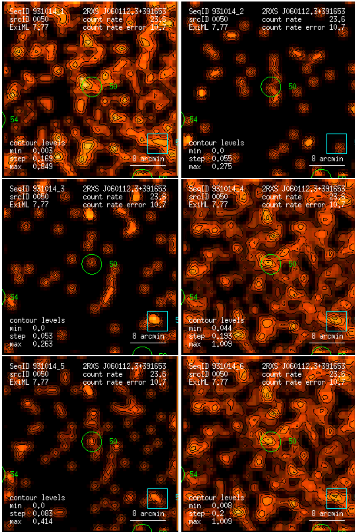
Figure 50: RASS 931014: detection 0050: band rate images, Gaussian filter: (1) PSPC channels 11 – 41, (2) 52 – 90, (3) 91 – 201, (4) 11 – 235, (5) 52 – 201, (6) 11 – 201. Broad band rates in counts/ks. Band rate contour levels in counts/ks/arcmin 2 .
