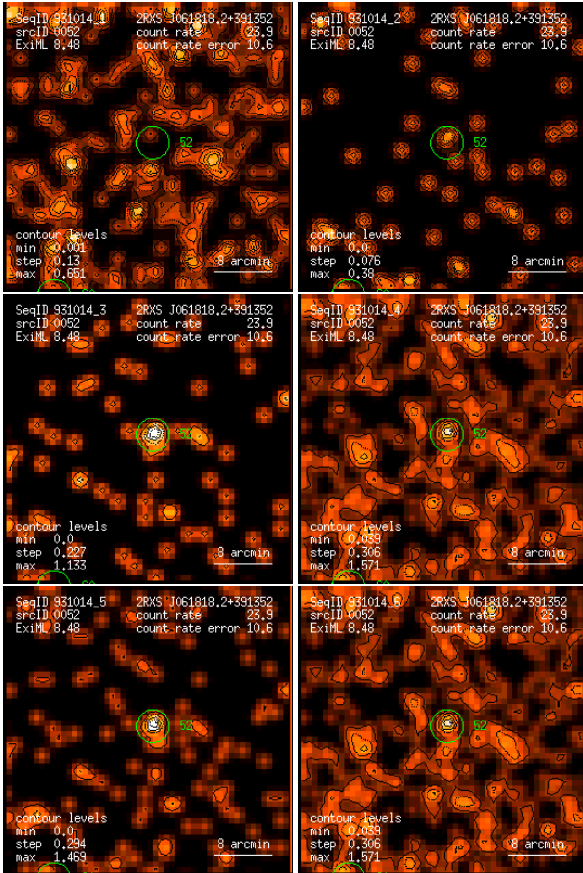
Figure 52: RASS 931014: detection 0052: band rate images, Gaussian filter: (1) PSPC channels 11 – 41, (2) 52 – 90, (3) 91 – 201, (4) 11 – 235, (5) 52 – 201, (6) 11 – 201. Broad band rates in counts/ks. Band rate contour levels in counts/ks/arcmin 2 .
