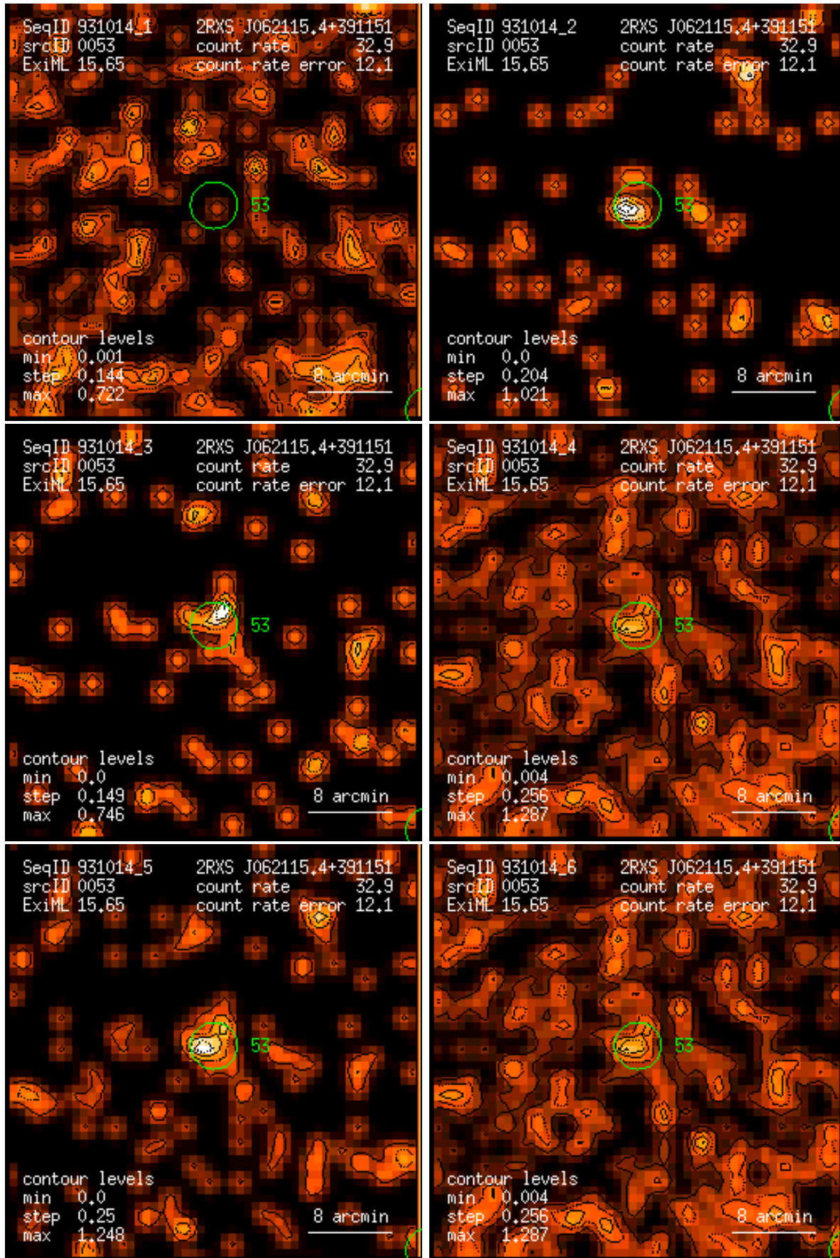
Figure 53: RASS 931014: detection 0053: band rate images, Gaussian filter: (1) PSPC channels 11 – 41, (2) 52 – 90, (3) 91 – 201, (4) 11 – 235, (5) 52 – 201, (6) 11 – 201. Broad band rates in counts/ks. Band rate contour levels in counts/ks/arcmin 2 .
