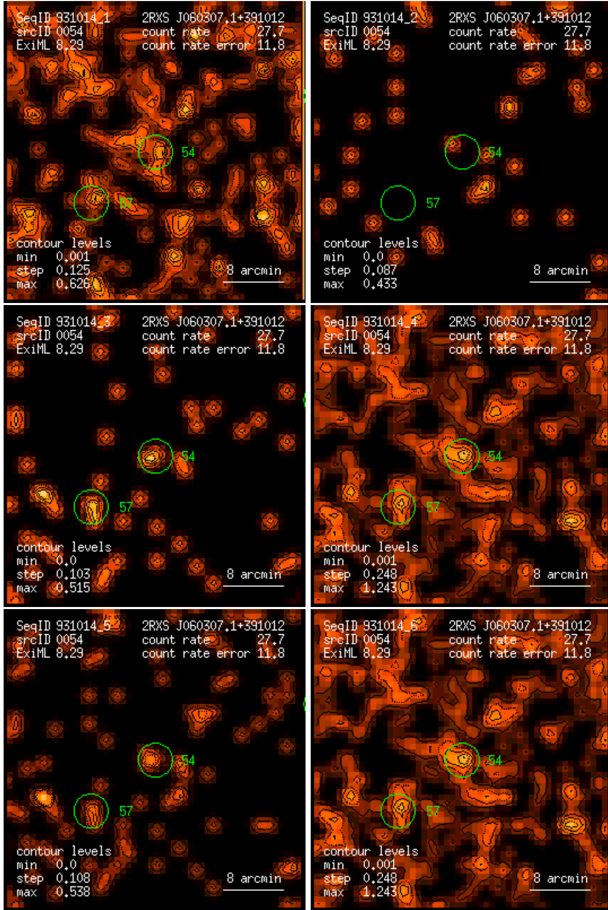
Figure 54: RASS 931014: detection 0054: band rate images, Gaussian filter: (1) PSPC channels 11 – 41, (2) 52 – 90, (3) 91 – 201, (4) 11 – 235, (5) 52 – 201, (6) 11 – 201. Broad band rates in counts/ks. Band rate contour levels in counts/ks/arcmin 2 .
