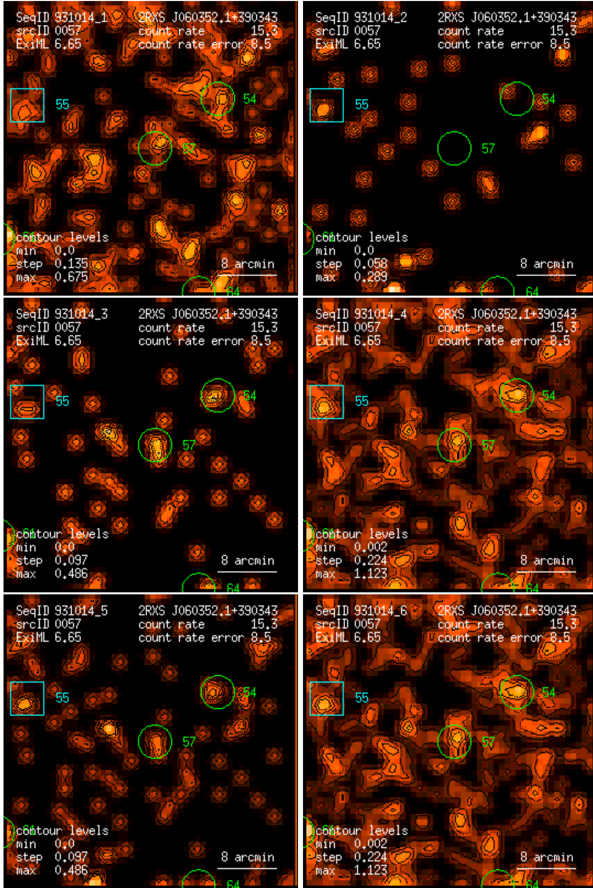
Figure 57: RASS 931014: detection 0057: band rate images, Gaussian filter: (1) PSPC channels 11 – 41, (2) 52 – 90, (3) 91 – 201, (4) 11 – 235, (5) 52 – 201, (6) 11 – 201. Broad band rates in counts/ks. Band rate contour levels in counts/ks/arcmin 2 .
