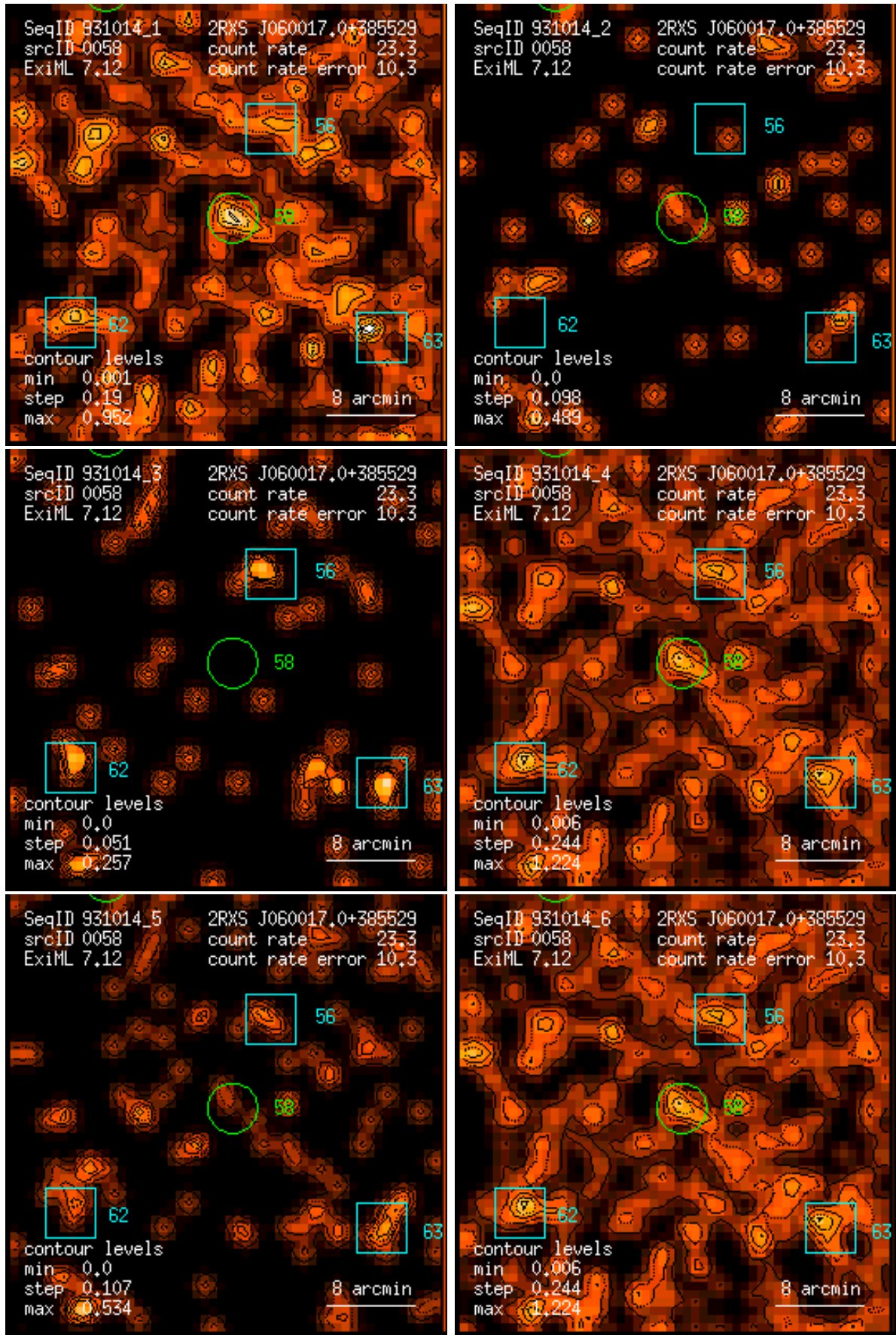
Figure 58: RASS 931014: detection 0058: band rate images, Gaussian filter: (1) PSPC channels 11 – 41, (2) 52 – 90, (3) 91 – 201, (4) 11 – 235, (5) 52 – 201, (6) 11 – 201. Broad band rates in counts/ks. Band rate contour levels in counts/ks/arcmin 2 .
