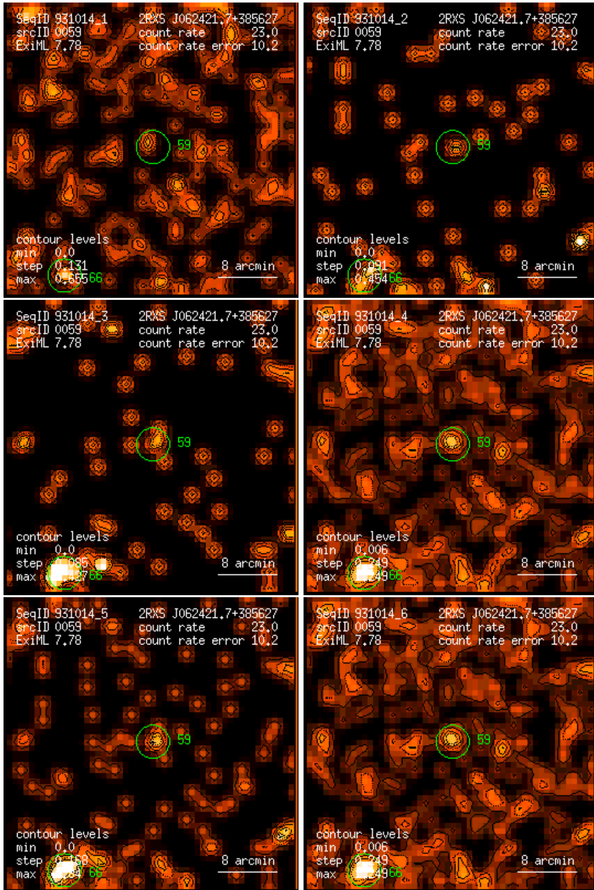
Figure 59: RASS 931014: detection 0059: band rate images, Gaussian filter: (1) PSPC channels 11 – 41, (2) 52 – 90, (3) 91 – 201, (4) 11 – 235, (5) 52 – 201, (6) 11 – 201. Broad band rates in counts/ks. Band rate contour levels in counts/ks/arcmin 2 .
