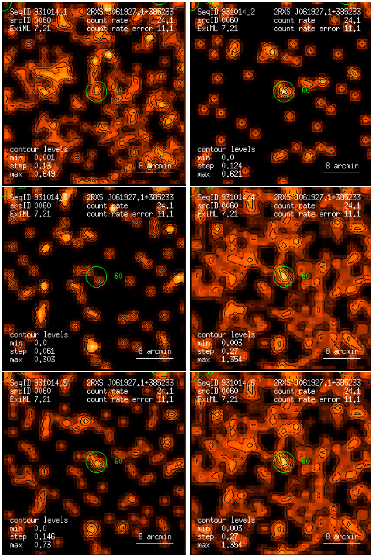
Figure 60: RASS 931014: detection 0060: band rate images, Gaussian filter: (1) PSPC channels 11 – 41, (2) 52 – 90, (3) 91 – 201, (4) 11 – 235, (5) 52 – 201, (6) 11 – 201. Broad band rates in counts/ks. Band rate contour levels in counts/ks/arcmin 2 .
