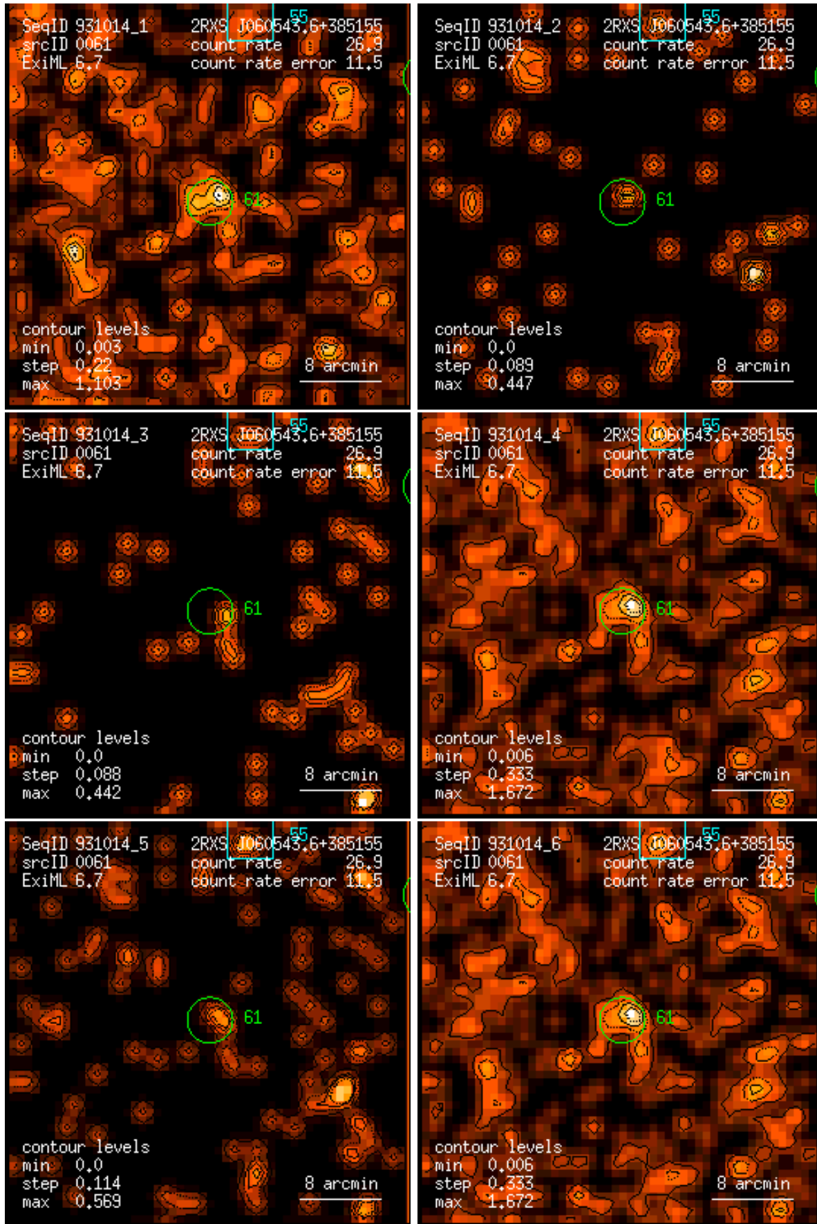
Figure 61: RASS 931014: detection 0061: band rate images, Gaussian filter: (1) PSPC channels 11 – 41, (2) 52 – 90, (3) 91 – 201, (4) 11 – 235, (5) 52 – 201, (6) 11 – 201. Broad band rates in counts/ks. Band rate contour levels in counts/ks/arcmin 2 .
