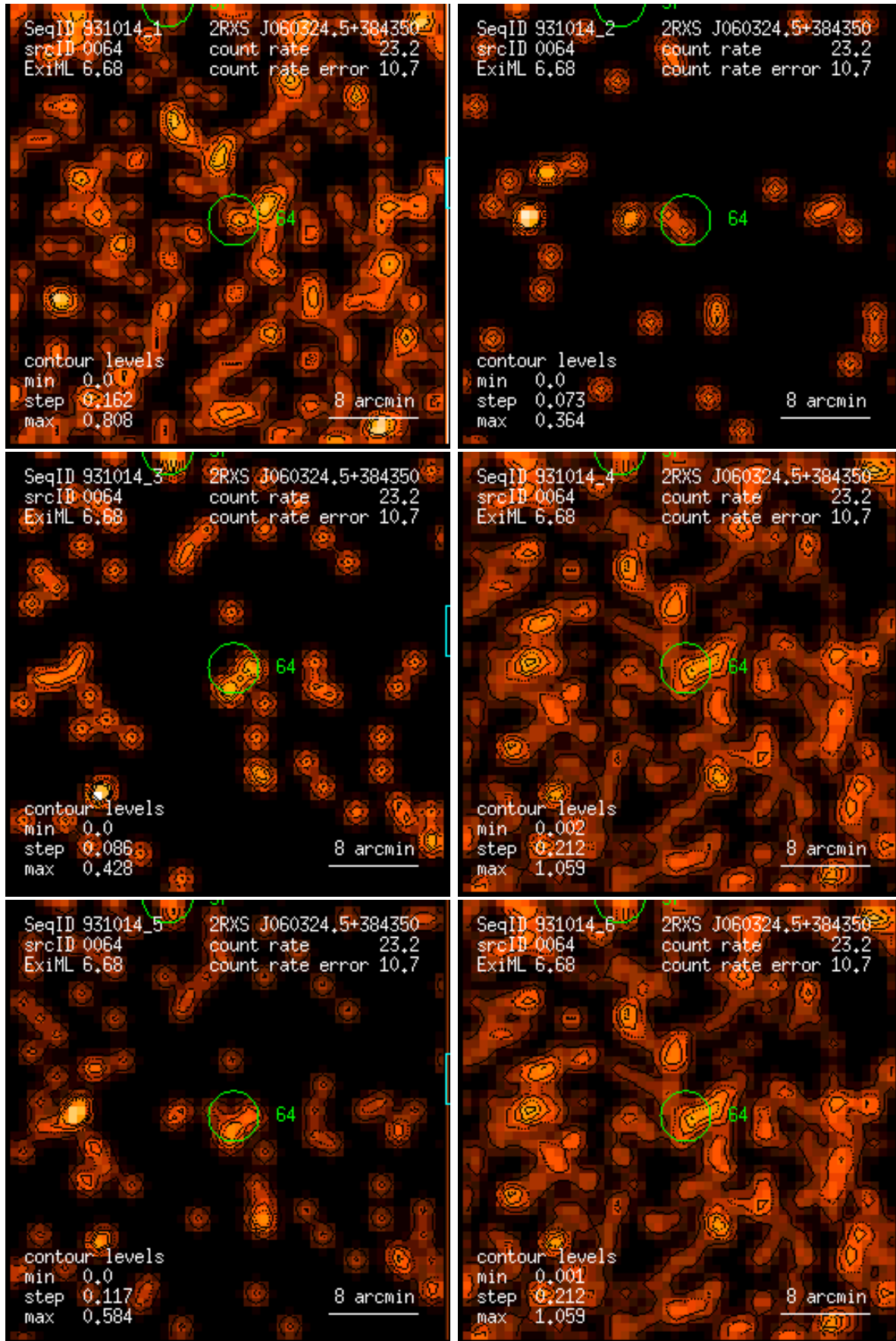
Figure 64: RASS 931014: detection 0064: band rate images, Gaussian filter: (1) PSPC channels 11 – 41, (2) 52 – 90, (3) 91 – 201, (4) 11 – 235, (5) 52 – 201, (6) 11 – 201. Broad band rates in counts/ks. Band rate contour levels in counts/ks/arcmin 2 .
