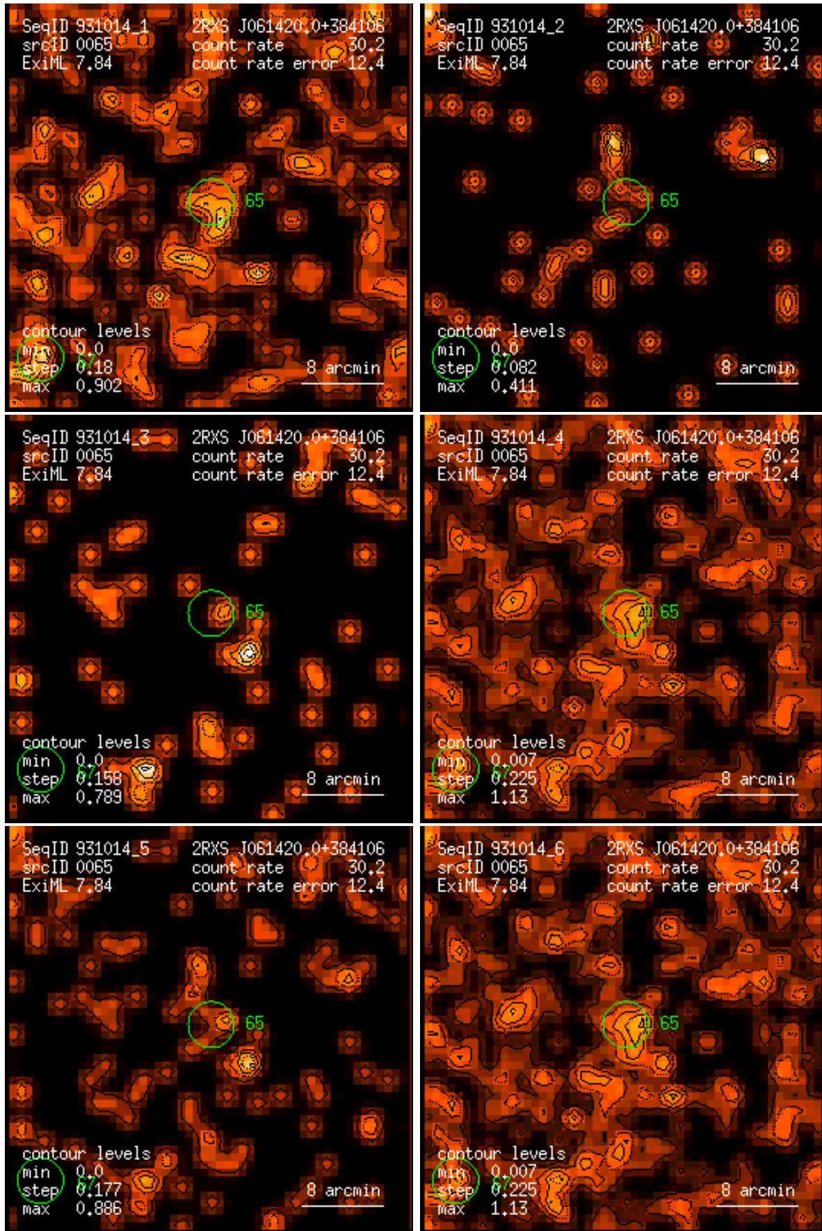
Figure 65: RASS 931014: detection 0065: band rate images, Gaussian filter: (1) PSPC channels 11 – 41, (2) 52 – 90, (3) 91 – 201, (4) 11 – 235, (5) 52 – 201, (6) 11 – 201. Broad band rates in counts/ks. Band rate contour levels in counts/ks/arcmin 2 .
