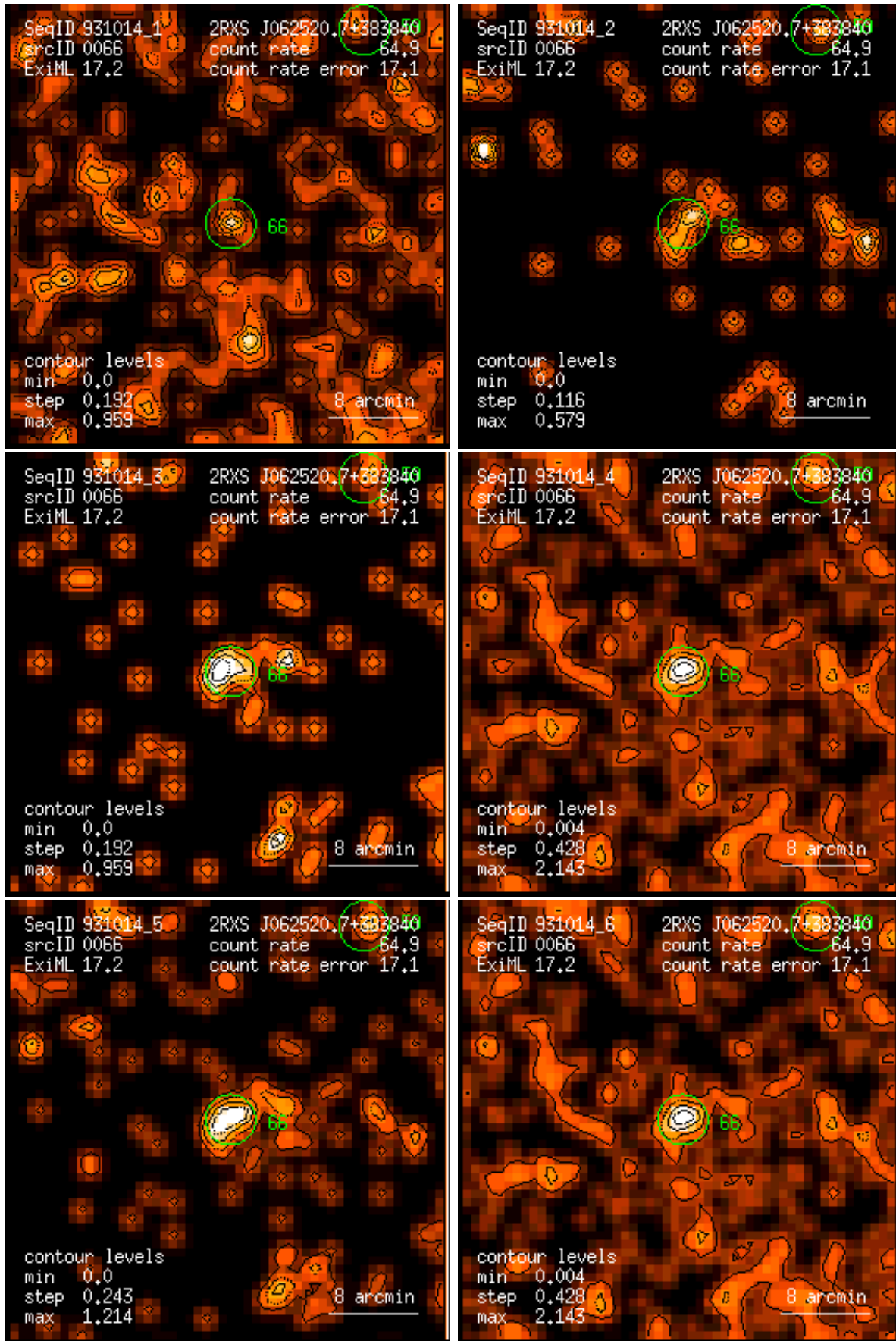
Figure 66: RASS 931014: detection 0066: band rate images, Gaussian filter: (1) PSPC channels 11 – 41, (2) 52 – 90, (3) 91 – 201, (4) 11 – 235, (5) 52 – 201, (6) 11 – 201. Broad band rates in counts/ks. Band rate contour levels in counts/ks/arcmin 2 .
