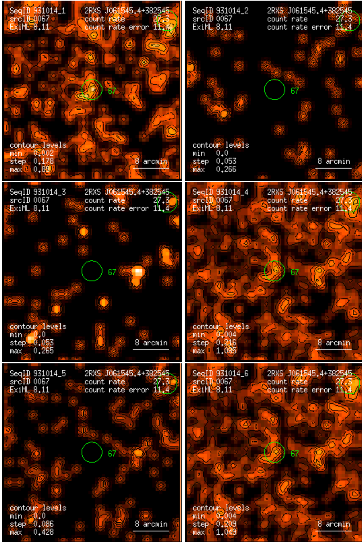
Figure 67: RASS 931014: detection 0067: band rate images, Gaussian filter: (1) PSPC channels 11 – 41, (2) 52 – 90, (3) 91 – 201, (4) 11 – 235, (5) 52 – 201, (6) 11 – 201. Broad band rates in counts/ks. Band rate contour levels in counts/ks/arcmin 2 .
