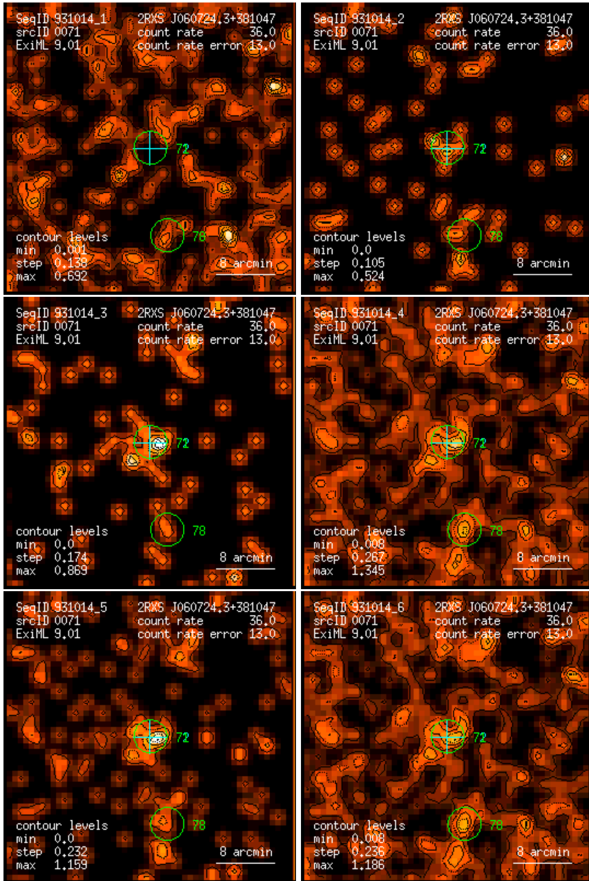
Figure 71: RASS 931014: detection 0071: band rate images, Gaussian filter: (1) PSPC channels 11 – 41, (2) 52 – 90, (3) 91 – 201, (4) 11 – 235, (5) 52 – 201, (6) 11 – 201. Broad band rates in counts/ks. Band rate contour levels in counts/ks/arcmin 2 .
