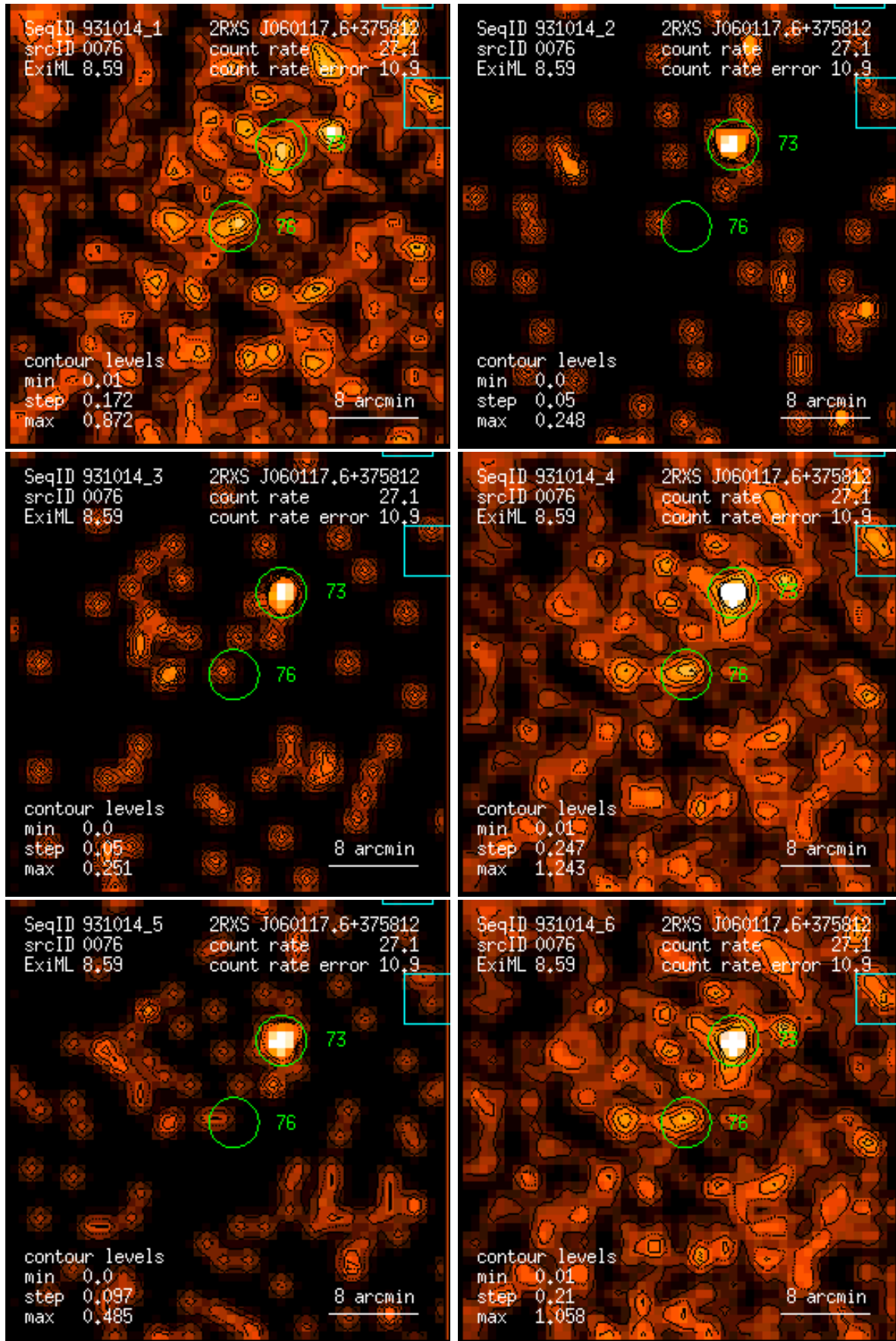
Figure 76: RASS 931014: detection 0076: band rate images, Gaussian filter: (1) PSPC channels 11 – 41, (2) 52 – 90, (3) 91 – 201, (4) 11 – 235, (5) 52 – 201, (6) 11 – 201. Broad band rates in counts/ks. Band rate contour levels in counts/ks/arcmin 2 .
