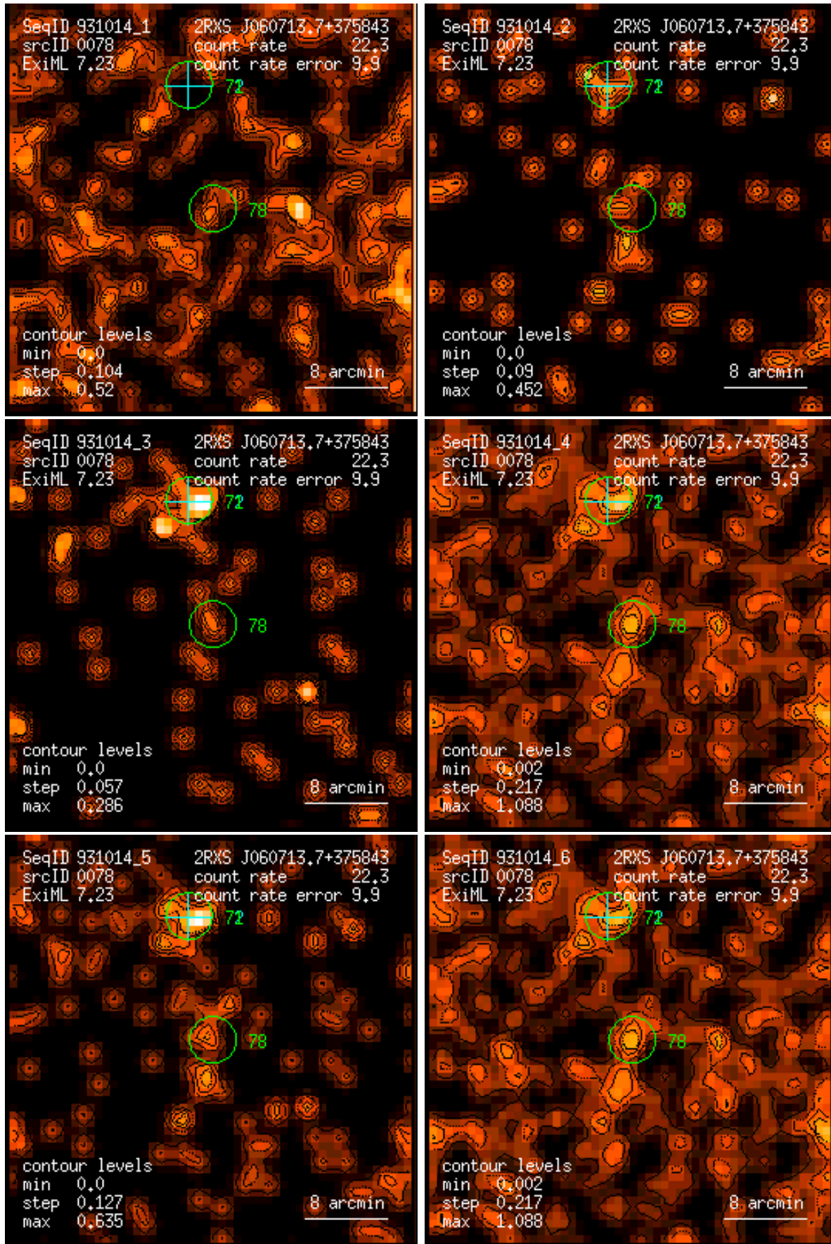
Figure 78: RASS 931014: detection 0078: band rate images, Gaussian filter: (1) PSPC channels 11 – 41, (2) 52 – 90, (3) 91 – 201, (4) 11 – 235, (5) 52 – 201, (6) 11 – 201. Broad band rates in counts/ks. Band rate contour levels in counts/ks/arcmin 2 .
