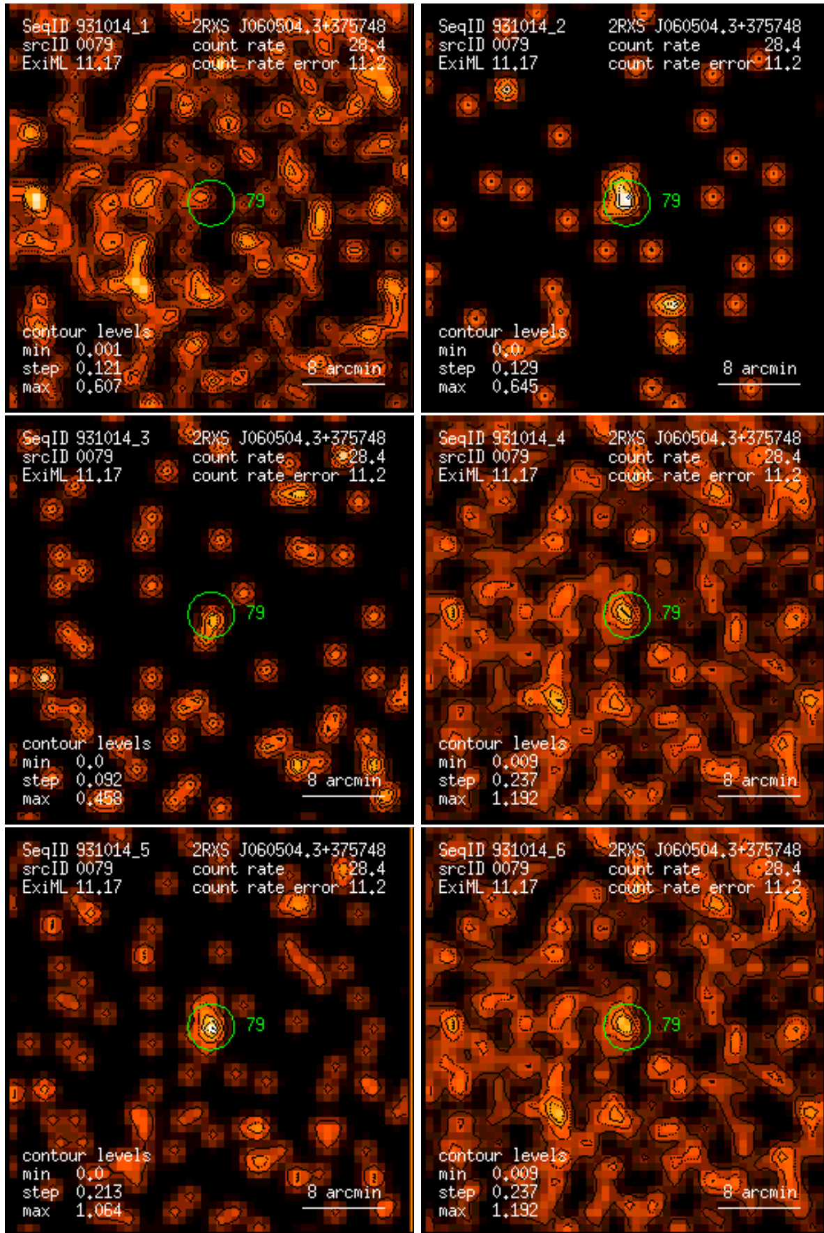
Figure 79: RASS 931014: detection 0079: band rate images, Gaussian filter: (1) PSPC channels 11 – 41, (2) 52 – 90, (3) 91 – 201, (4) 11 – 235, (5) 52 – 201, (6) 11 – 201. Broad band rates in counts/ks. Band rate contour levels in counts/ks/arcmin 2 .
