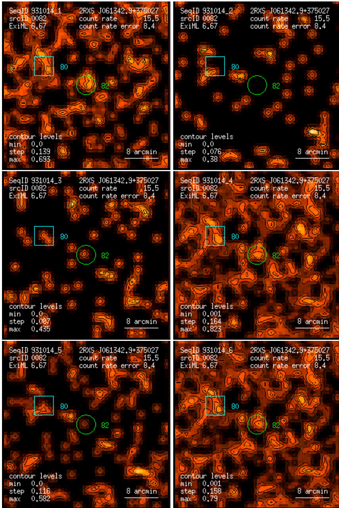
Figure 82: RASS 931014: detection 0082: band rate images, Gaussian filter: (1) PSPC channels 11 – 41, (2) 52 – 90, (3) 91 – 201, (4) 11 – 235, (5) 52 – 201, (6) 11 – 201. Broad band rates in counts/ks. Band rate contour levels in counts/ks/arcmin 2 .
