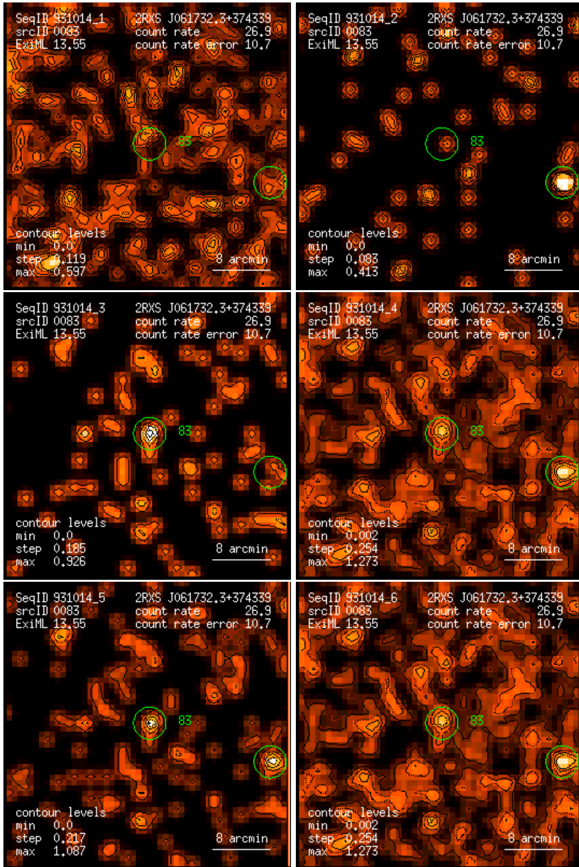
Figure 83: RASS 931014: detection 0083: band rate images, Gaussian filter: (1) PSPC channels 11 – 41, (2) 52 – 90, (3) 91 – 201, (4) 11 – 235, (5) 52 – 201, (6) 11 – 201. Broad band rates in counts/ks. Band rate contour levels in counts/ks/arcmin 2 .
