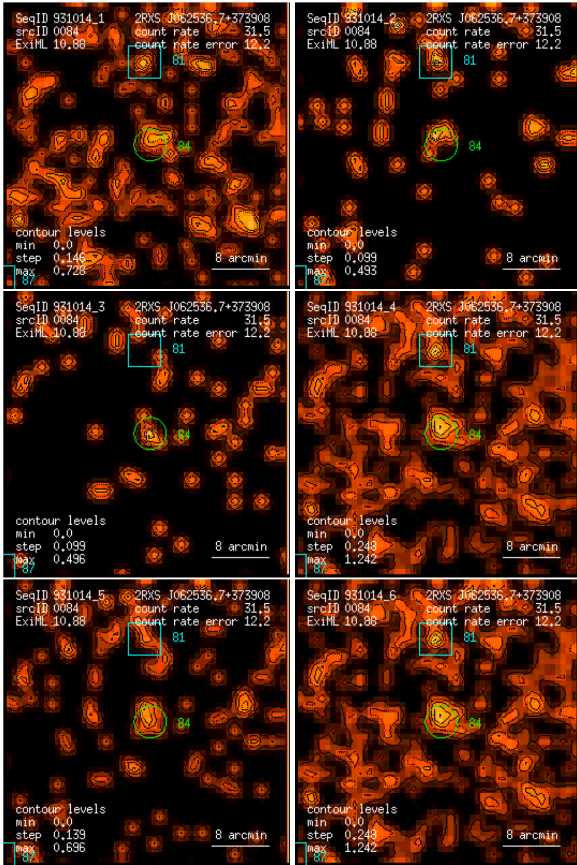
Figure 84: RASS 931014: detection 0084: band rate images, Gaussian filter: (1) PSPC channels 11 – 41, (2) 52 – 90, (3) 91 – 201, (4) 11 – 235, (5) 52 – 201, (6) 11 – 201. Broad band rates in counts/ks. Band rate contour levels in counts/ks/arcmin 2 .
