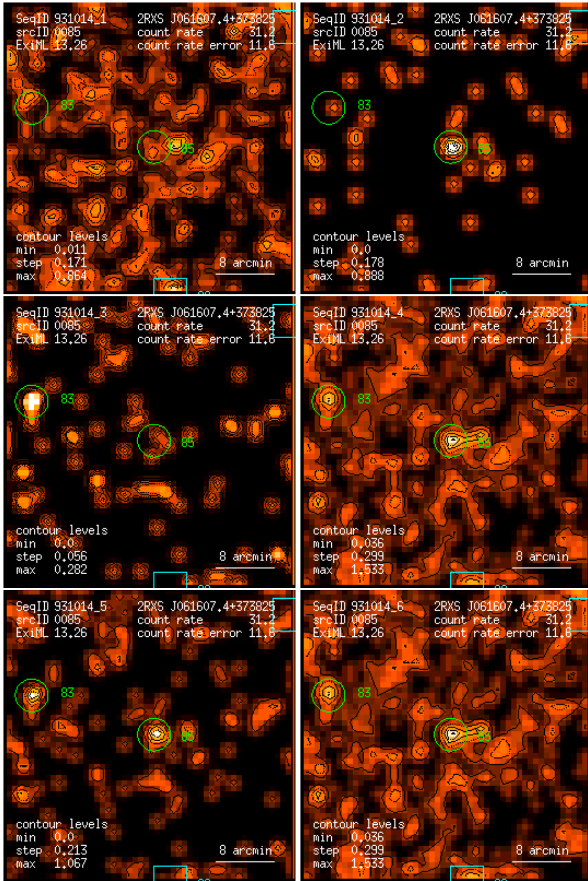
Figure 85: RASS 931014: detection 0085: band rate images, Gaussian filter: (1) PSPC channels 11 – 41, (2) 52 – 90, (3) 91 – 201, (4) 11 – 235, (5) 52 – 201, (6) 11 – 201. Broad band rates in counts/ks. Band rate contour levels in counts/ks/arcmin 2 .
