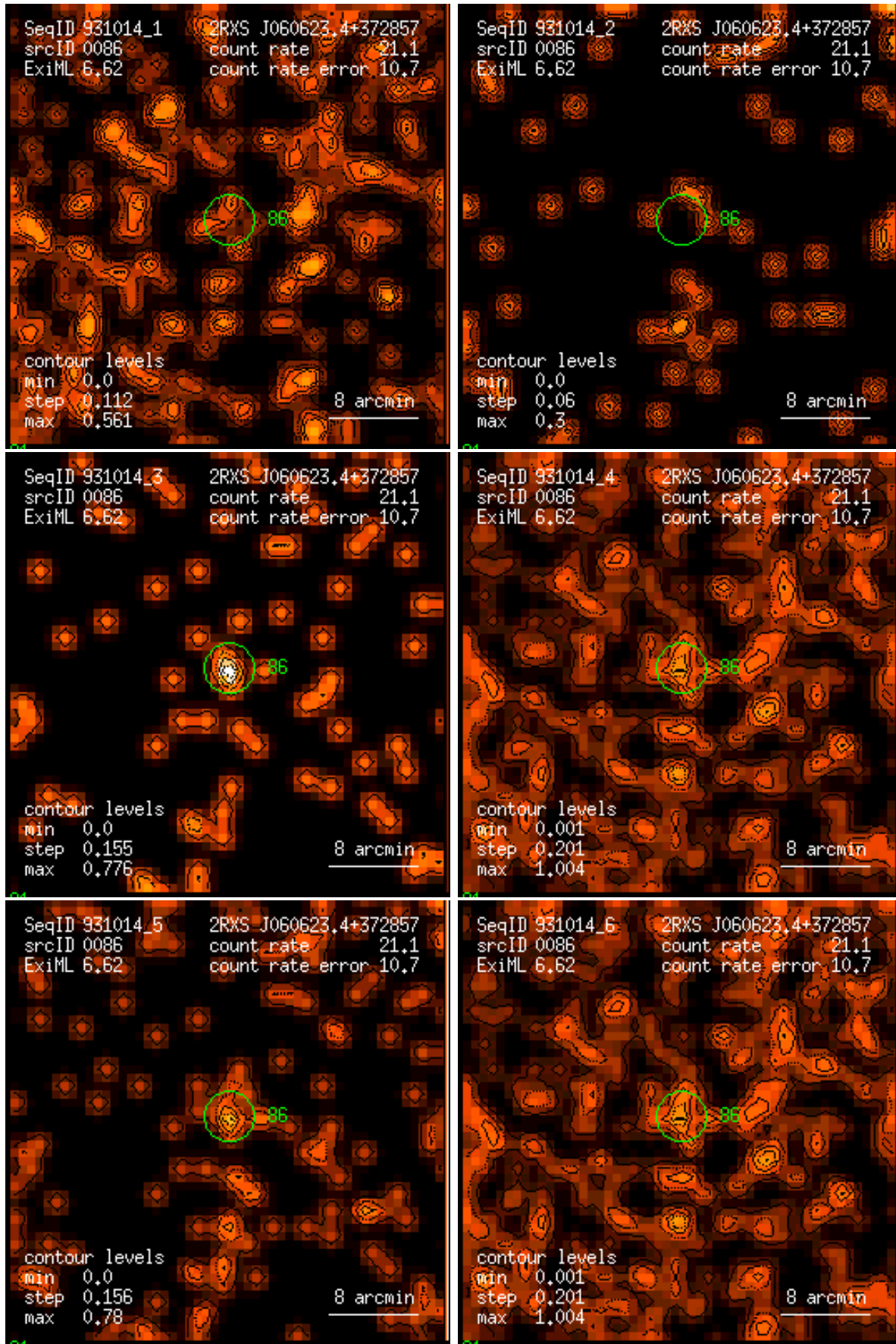
Figure 86: RASS 931014: detection 0086: band rate images, Gaussian filter: (1) PSPC channels 11 – 41, (2) 52 – 90, (3) 91 – 201, (4) 11 – 235, (5) 52 – 201, (6) 11 – 201. Broad band rates in counts/ks. Band rate contour levels in counts/ks/arcmin 2 .
