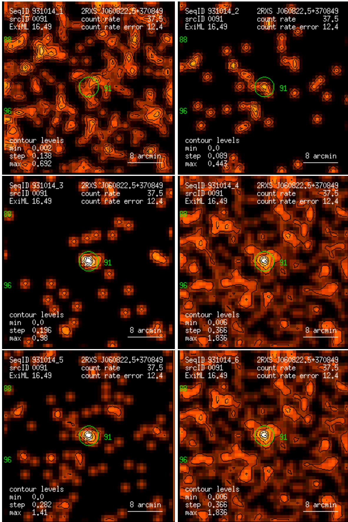
Figure 91: RASS 931014: detection 0091: band rate images, Gaussian filter: (1) PSPC channels 11 – 41, (2) 52 – 90, (3) 91 – 201, (4) 11 – 235, (5) 52 – 201, (6) 11 – 201. Broad band rates in counts/ks. Band rate contour levels in counts/ks/arcmin 2 .
