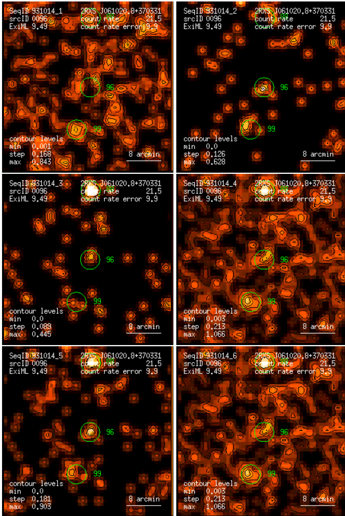
Figure 96: RASS 931014: detection 0096: band rate images, Gaussian filter: (1) PSPC channels 11 – 41, (2) 52 – 90, (3) 91 – 201, (4) 11 – 235, (5) 52 – 201, (6) 11 – 201. Broad band rates in counts/ks. Band rate contour levels in counts/ks/arcmin 2 .
