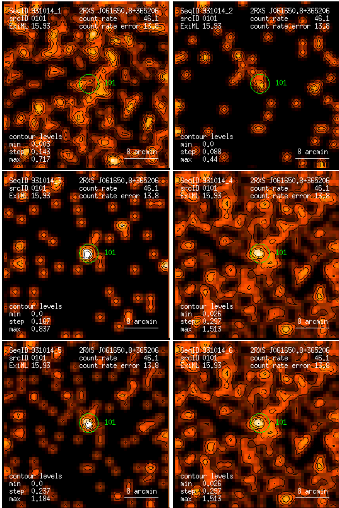
Figure 101: RASS 931014: detection 0101: band rate images, Gaussian filter: (1) PSPC channels 11 – 41, (2) 52 – 90, (3) 91 – 201, (4) 11 – 235, (5) 52 – 201, (6) 11 – 201. Broad band rates in counts/ks. Band rate contour levels in counts/ks/arcmin 2 .
