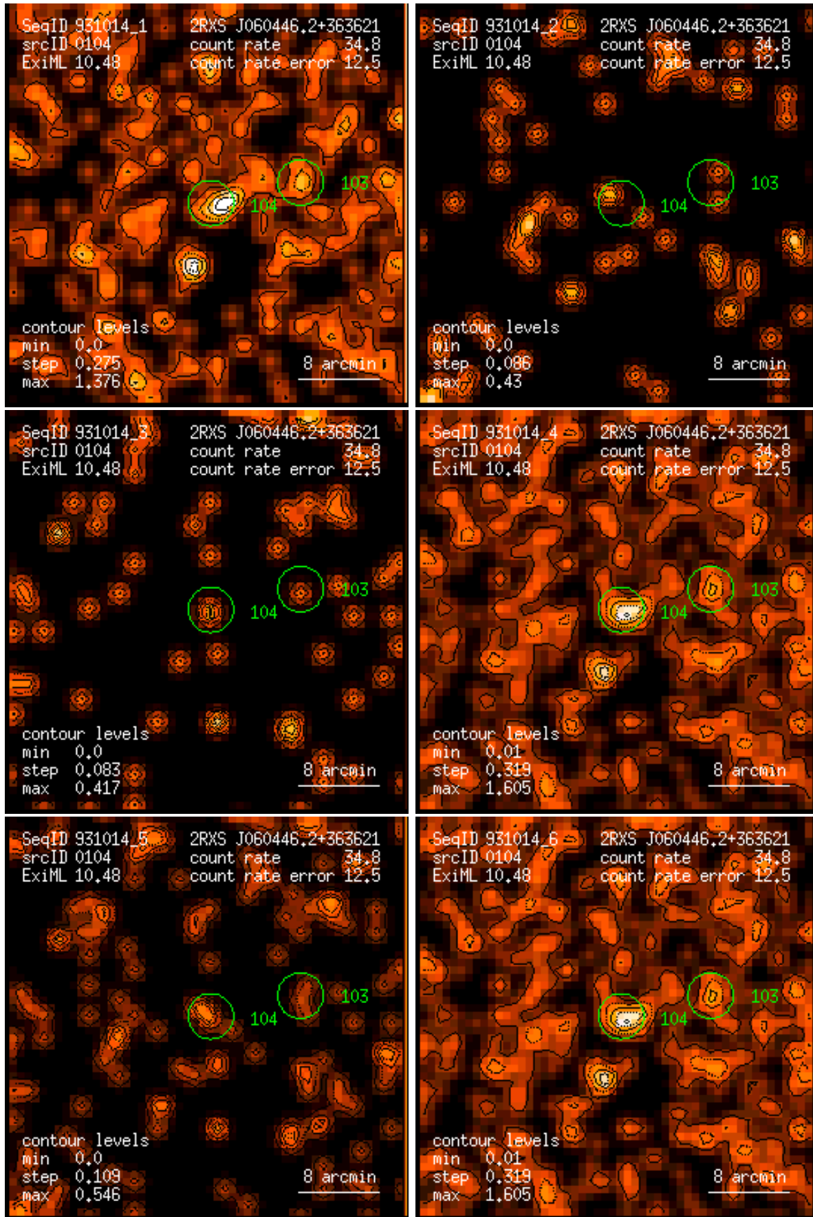
Figure 104: RASS 931014: detection 0104: band rate images, Gaussian filter: (1) PSPC channels 11 – 41, (2) 52 – 90, (3) 91 – 201, (4) 11 – 235, (5) 52 – 201, (6) 11 – 201. Broad band rates in counts/ks. Band rate contour levels in counts/ks/arcmin 2 .
