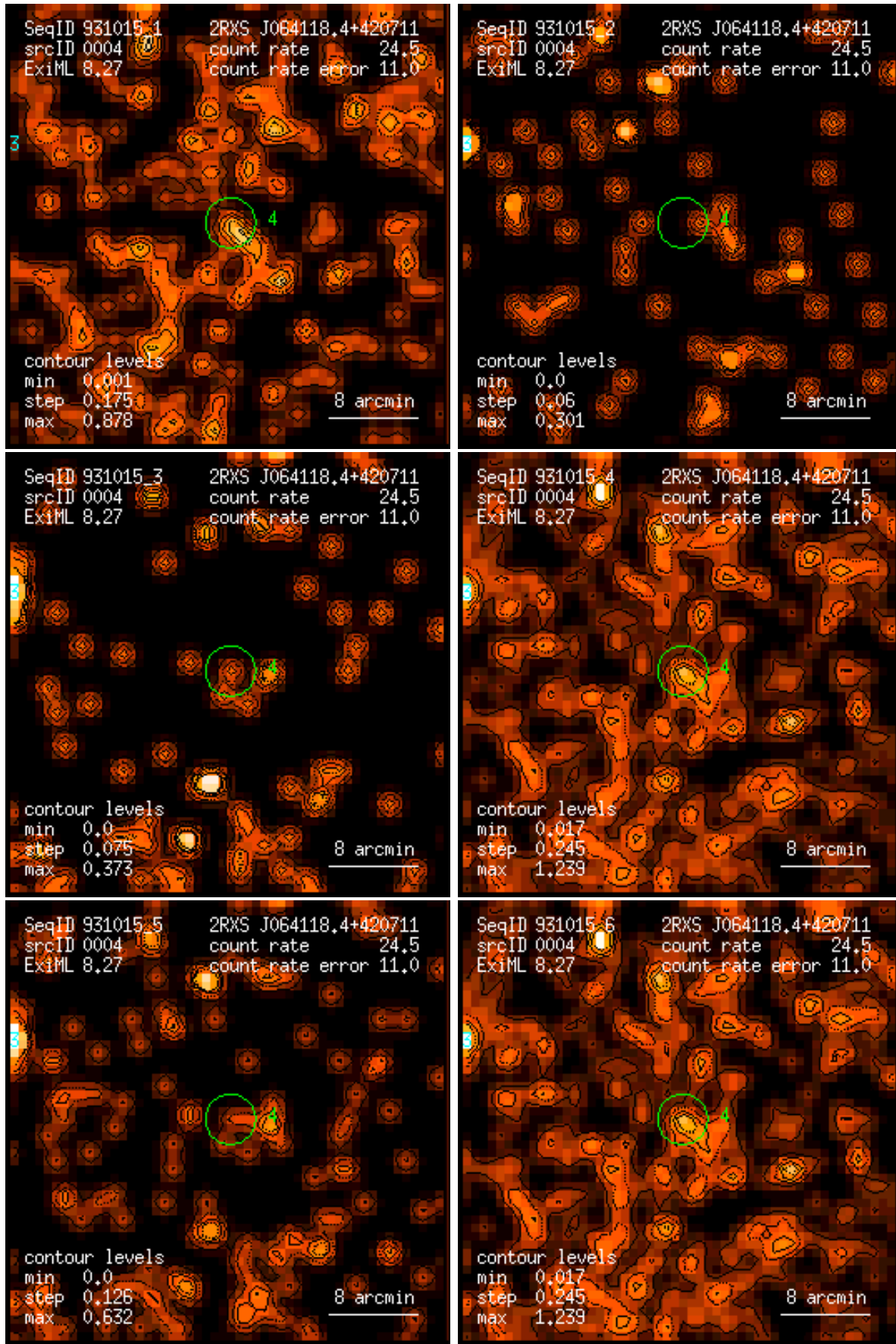
Figure 4: RASS 931015: detection 0004: band rate images, Gaussian filter: (1) PSPC channels 11 – 41, (2) 52 – 90, (3) 91 – 201, (4) 11 – 235, (5) 52 – 201, (6) 11 – 201. Broad band rates in counts/ks. Band rate contour levels in counts/ks/arcmin 2 .
