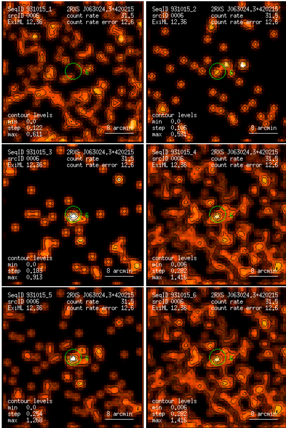
Figure 6: RASS 931015: detection 0006: band rate images, Gaussian filter: (1) PSPC channels 11 – 41, (2) 52 – 90, (3) 91 – 201, (4) 11 – 235, (5) 52 – 201, (6) 11 – 201. Broad band rates in counts/ks. Band rate contour levels in counts/ks/arcmin 2 .
