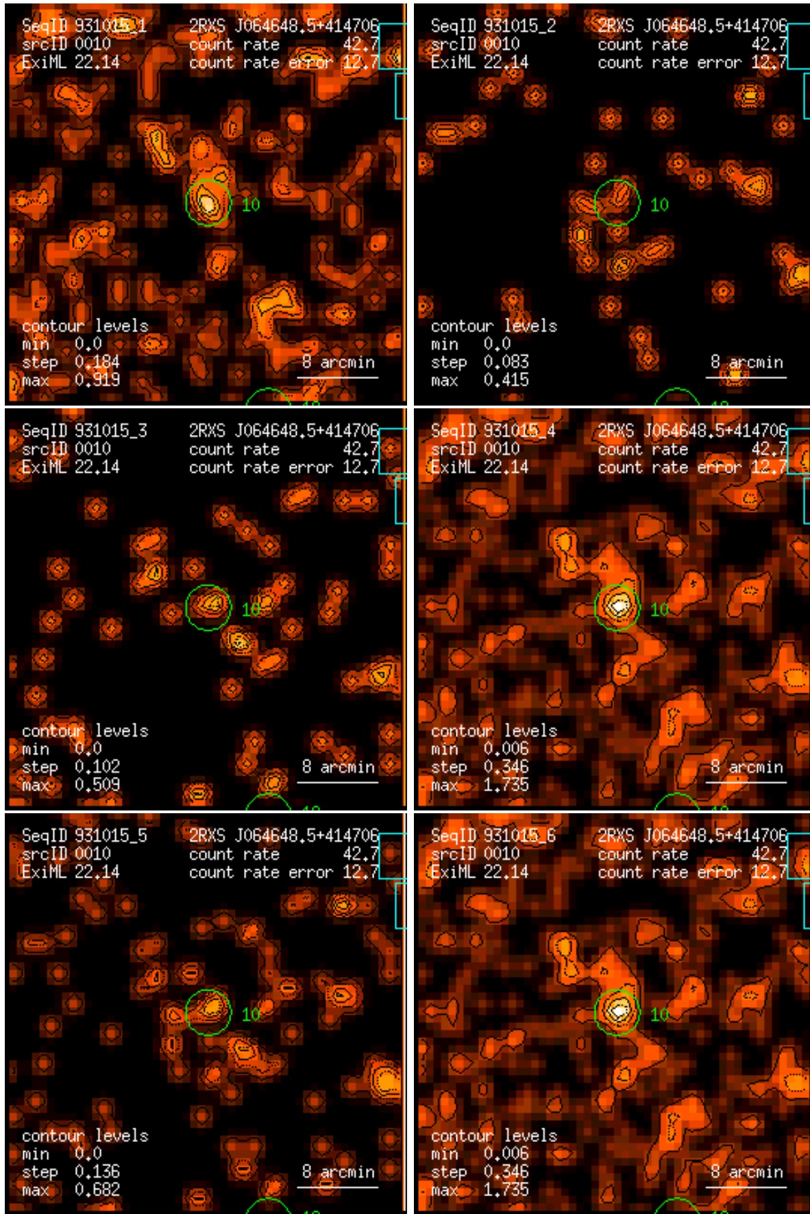
Figure 10: RASS 931015: detection 0010: band rate images, Gaussian filter: (1) PSPC channels 11 – 41, (2) 52 – 90, (3) 91 – 201, (4) 11 – 235, (5) 52 – 201, (6) 11 – 201. Broad band rates in counts/ks. Band rate contour levels in counts/ks/arcmin 2 .
