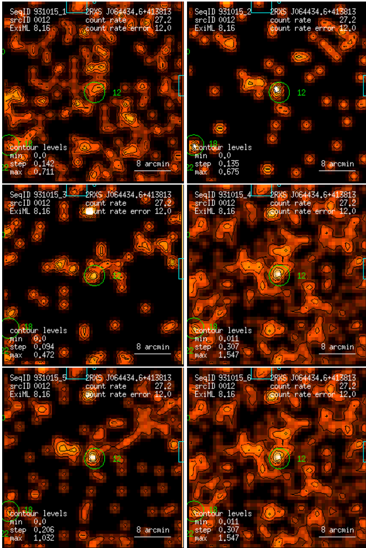
Figure 12: RASS 931015: detection 0012: band rate images, Gaussian filter: (1) PSPC channels 11 – 41, (2) 52 – 90, (3) 91 – 201, (4) 11 – 235, (5) 52 – 201, (6) 11 – 201. Broad band rates in counts/ks. Band rate contour levels in counts/ks/arcmin 2 .
